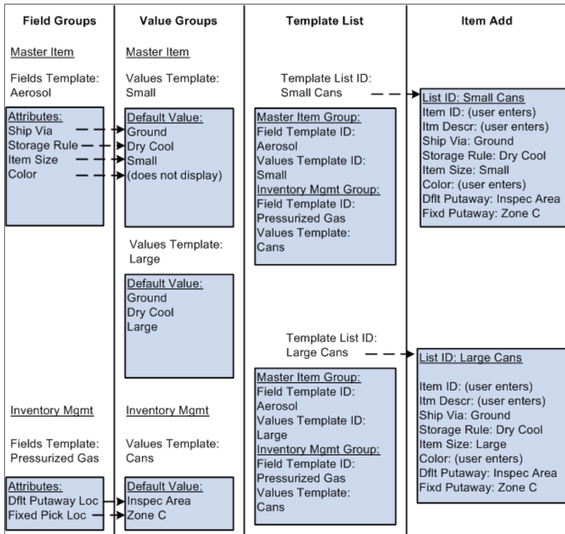
Example of Configurable Item Templates
