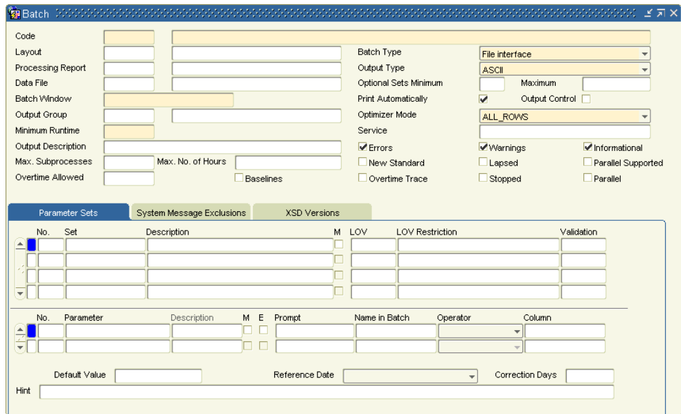
Figure 29: Batch definition
