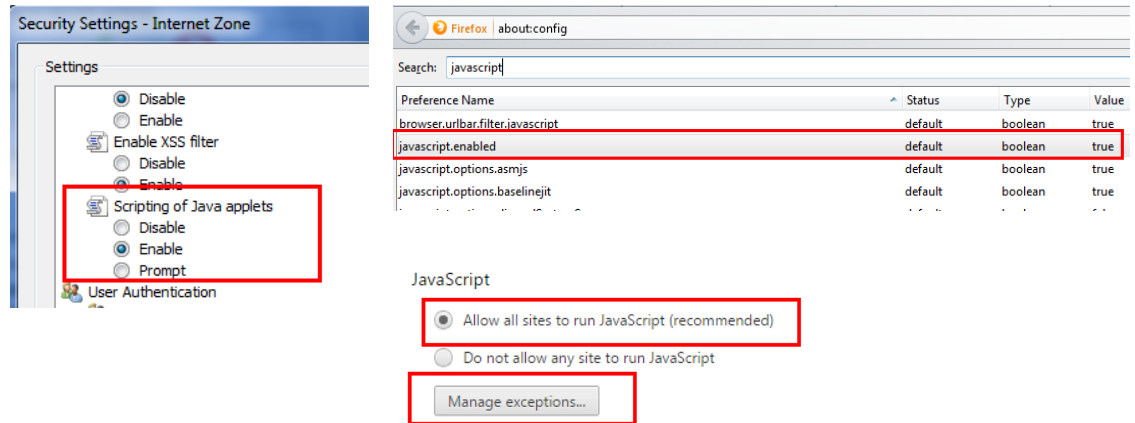
Figure 15 – Javascript Settings
