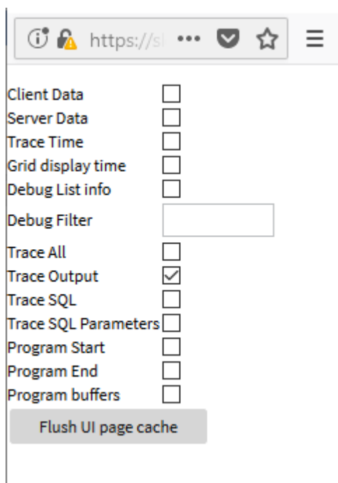
Figure 6 – Debug controls
