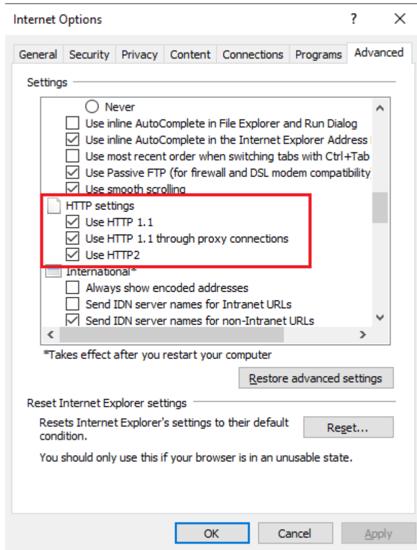
Figure 14 – HTTP 1.1 Settings
