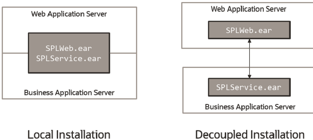
Figure 19 – Installation Modes
