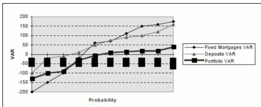
Graph for Output From Monte Carlo
