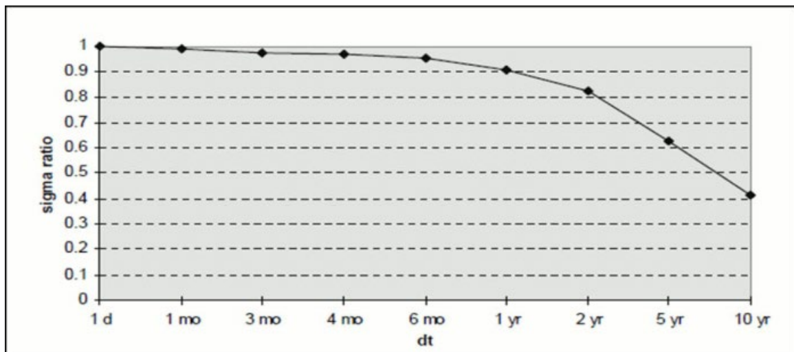
Graph of change in the ratio \sigma_{1m} / \sigma_{\text{varying } Dt} ( \alpha = 0.1 )
