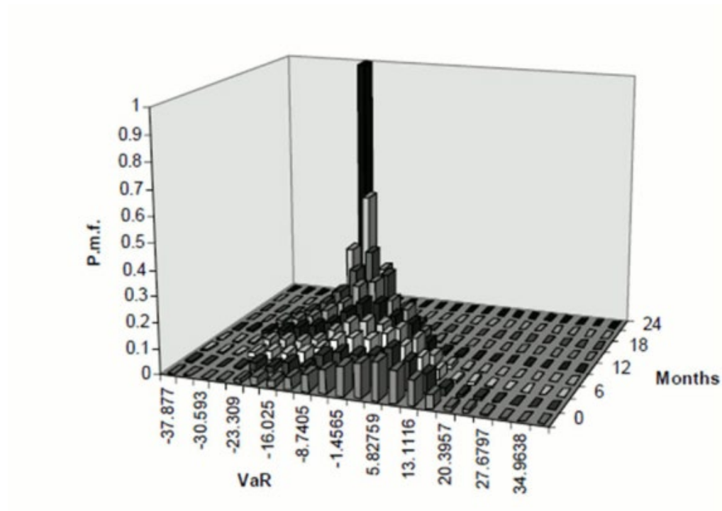
Graph of probability mass function
