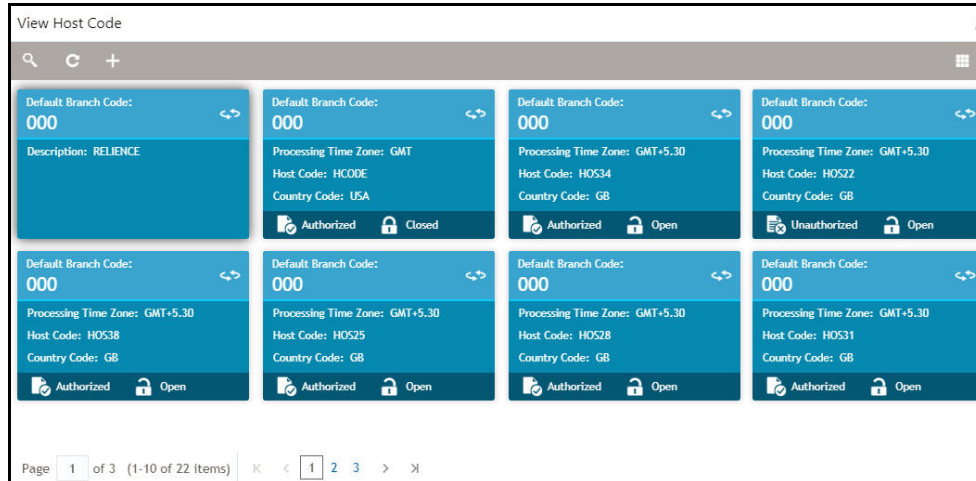
Figure 1.10: Flip View
