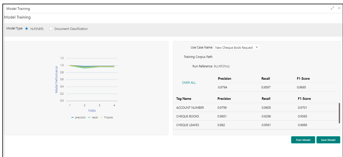
Figure 71: Model Training
