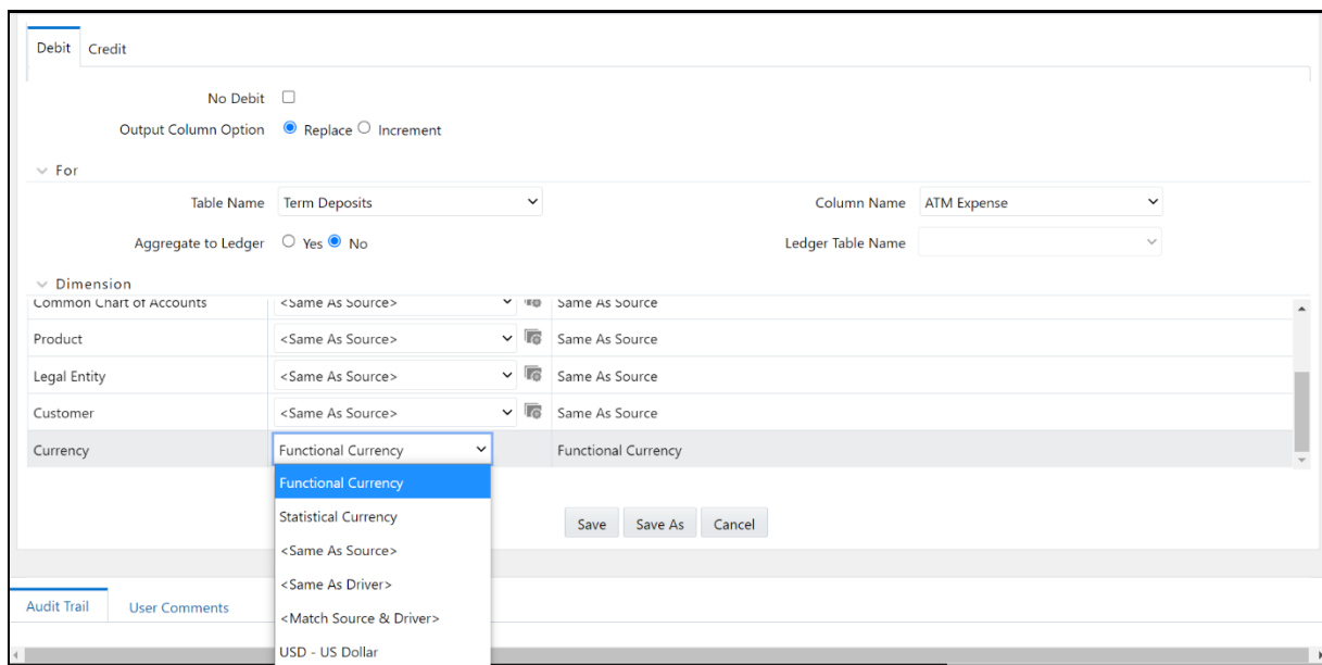
Figure 143: Output Tab Showing Multi-currency Options for a Dynamic Driver Rule
