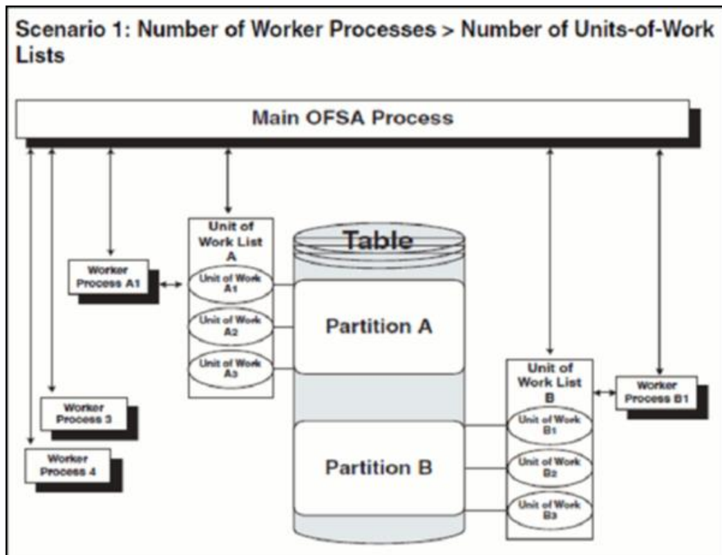
Figure 357: Number of Worker Processes greater than Number of Units-of-Work Lists
