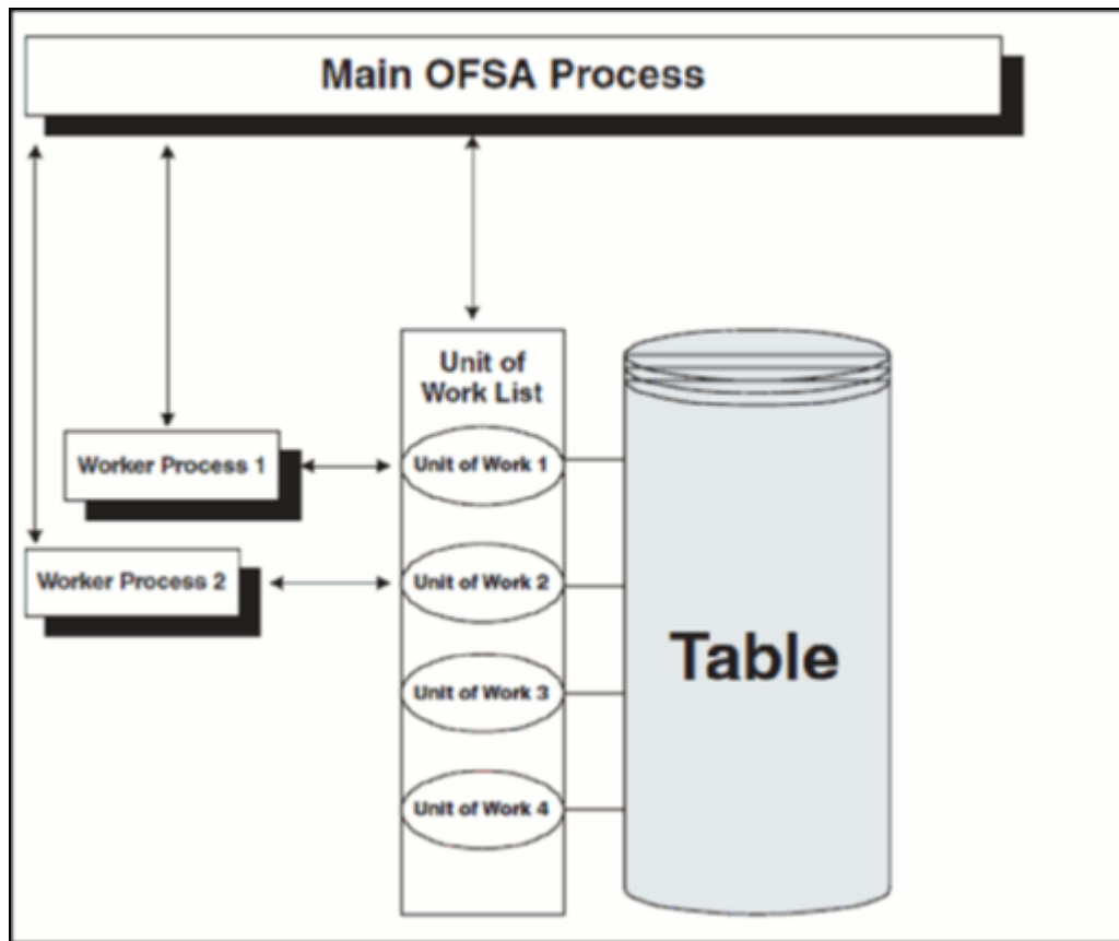
Figure 355: Main OFSAA Process
