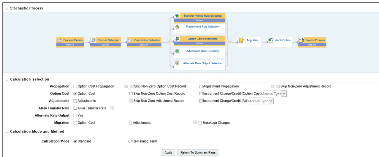
Figure 247: Stochastic Process - Calculation Selection
