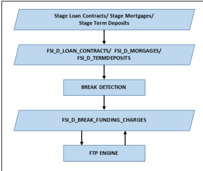
Figure 116: Break Identification Process Flow
