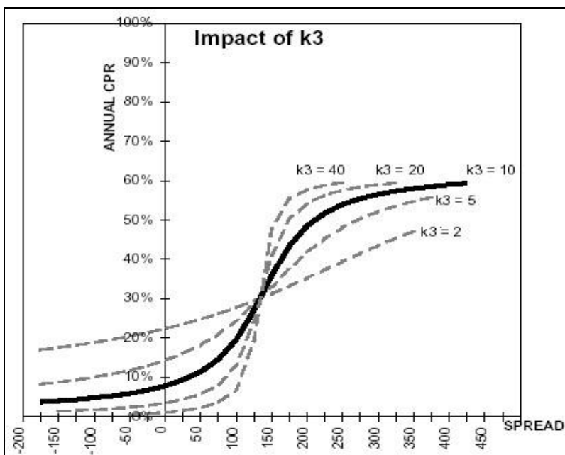
Figure 95: Impact of K3 on the Prepayment Curve
