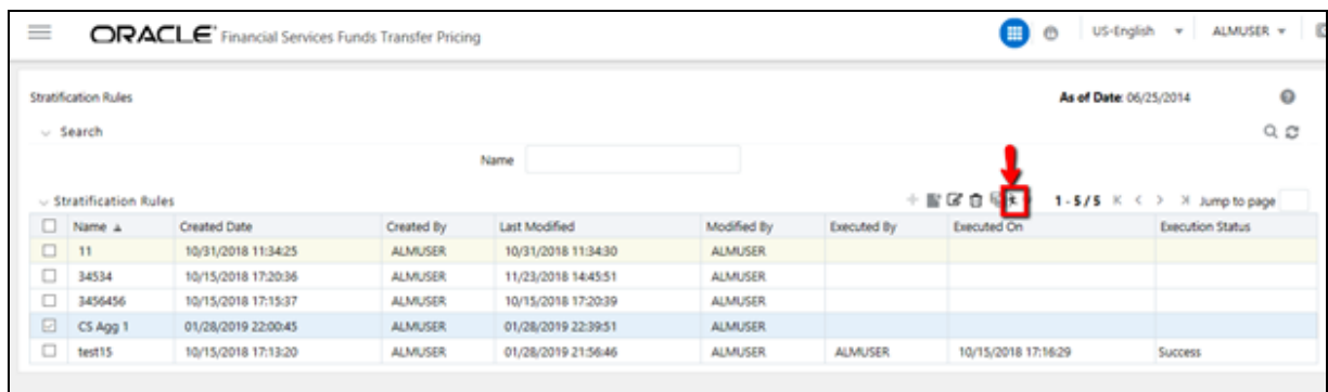
Figure 322: Stratification Rules
