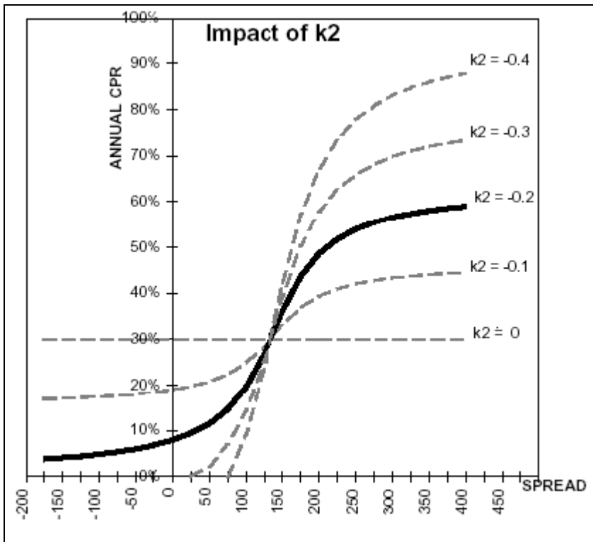
Figure 94: Impact of K2 on the Prepayment Curve
