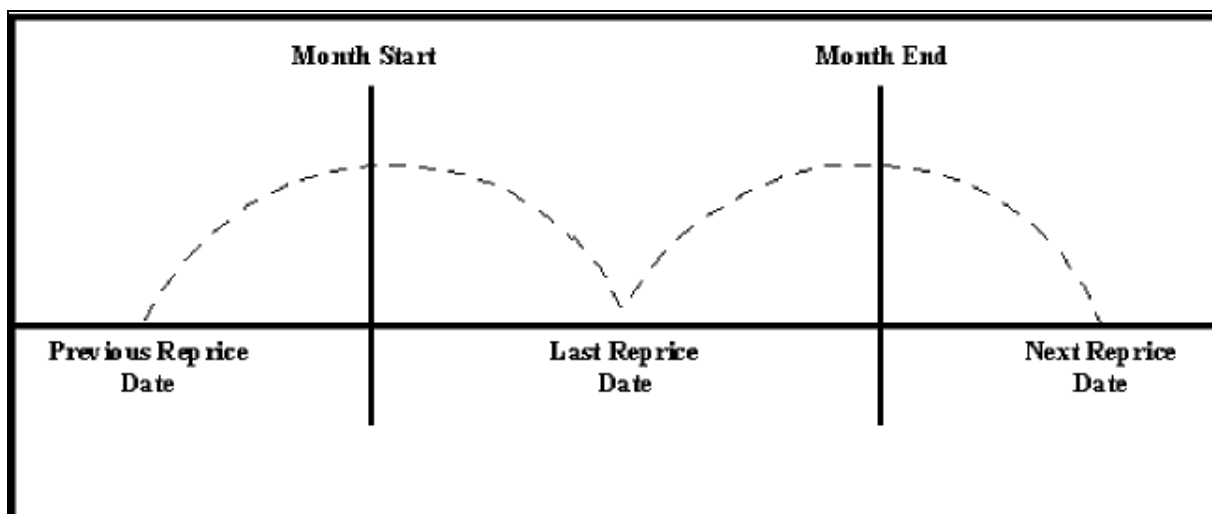
Figure 83: Mid-Period Repricing
