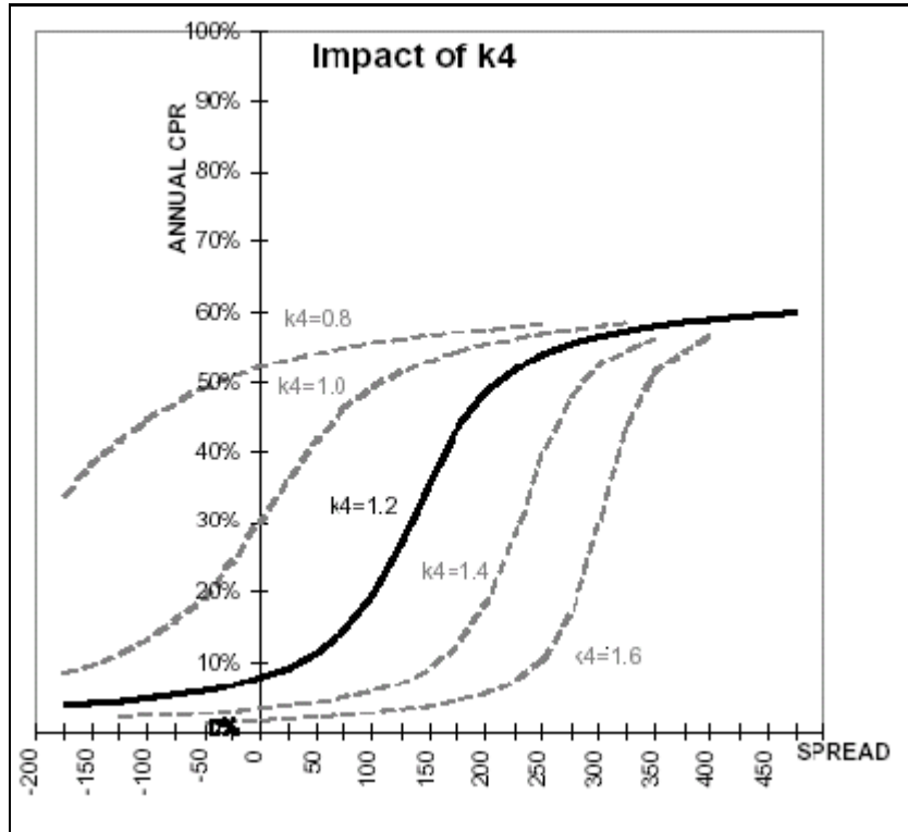
Figure 96: Impact of K4 on the Prepayment Curve
