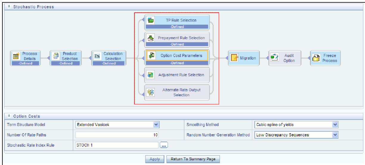
Figure 249: Stochastic Process - Rule Selection
