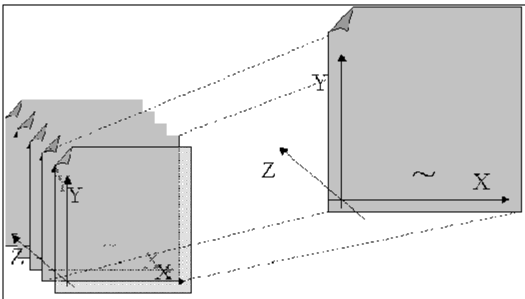
Figure 91: Three-Driver Prepayment Model
