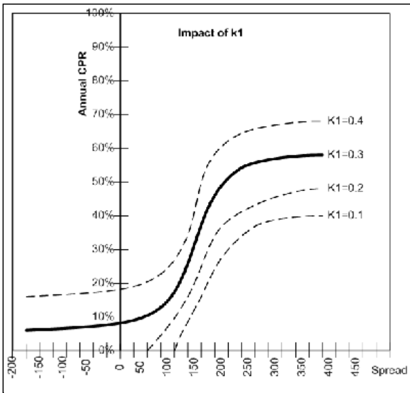
Figure 93: Impact of K_1 on the Prepayment Curve
