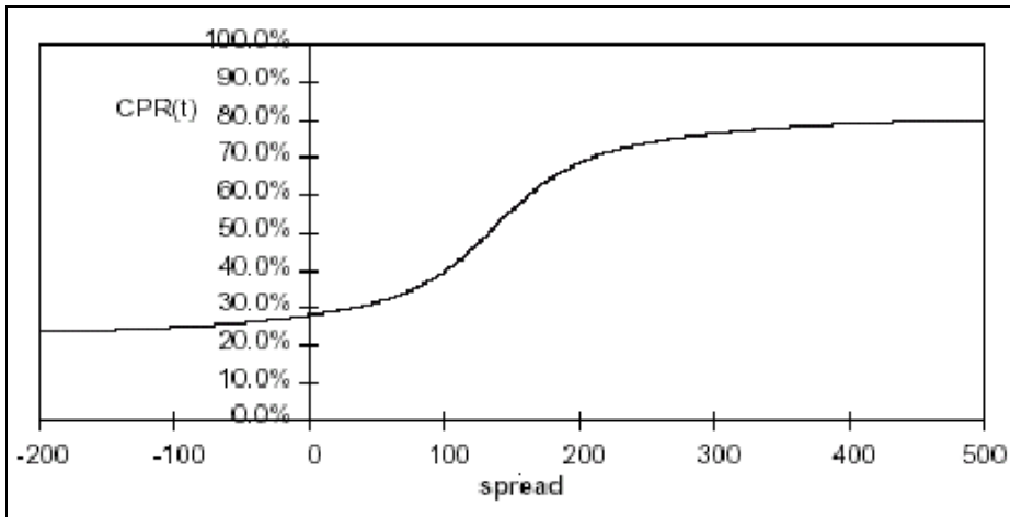
Figure 67: Prepayment Curve
