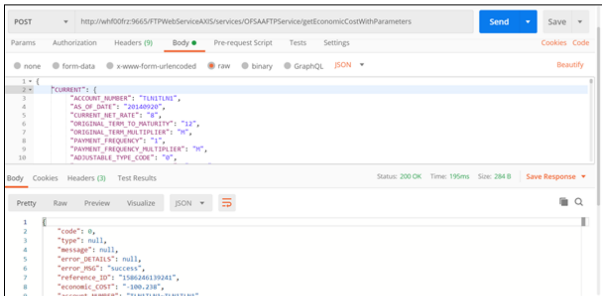
Figure 269: Web API Testing Tool (example Postman)
