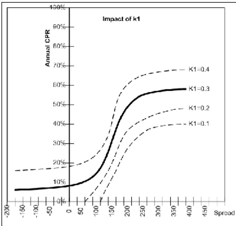
Figure 68: Impact of K_1 on the Prepayment Curve
