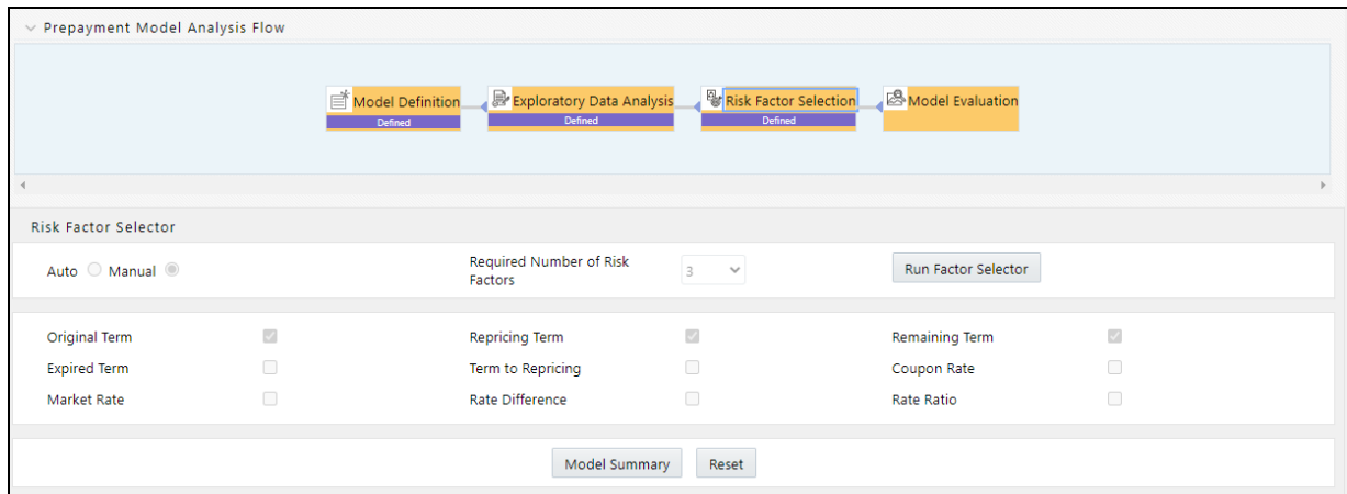
Figure 136: Prepayment Model Analysis – Risk Factor Selection tab
