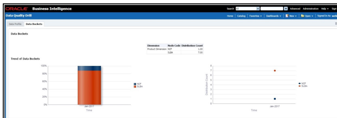
Figure 174: Data Bucket
