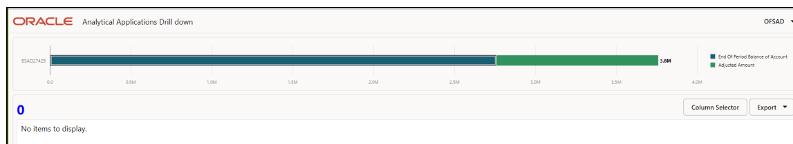
Figure 298: AgileREPORTER Drill-down
