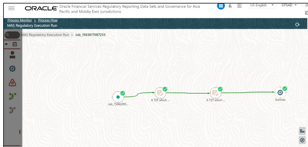
Figure 259: Execution Logs
