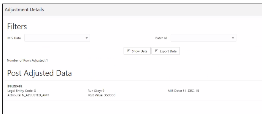
Figure 150: Adjustment Details
