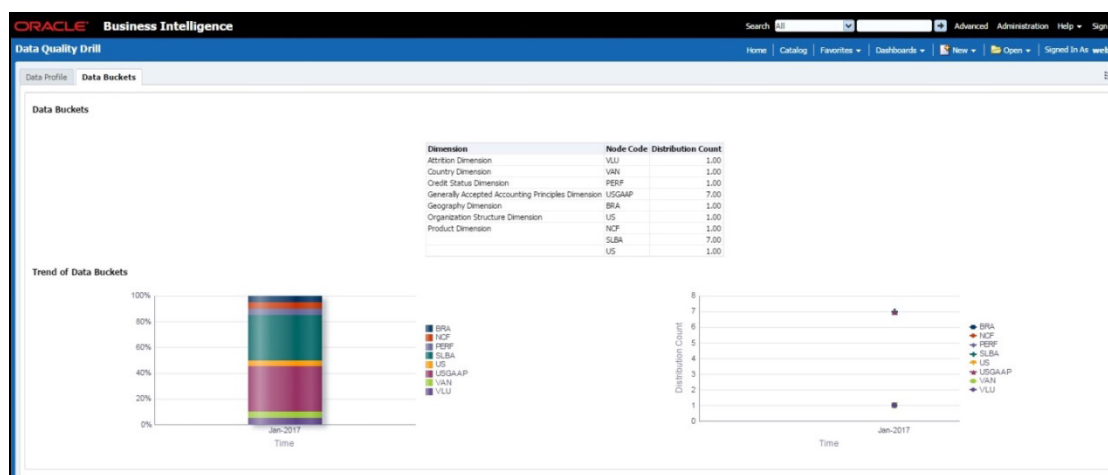
Figure 177: Data Buckets
