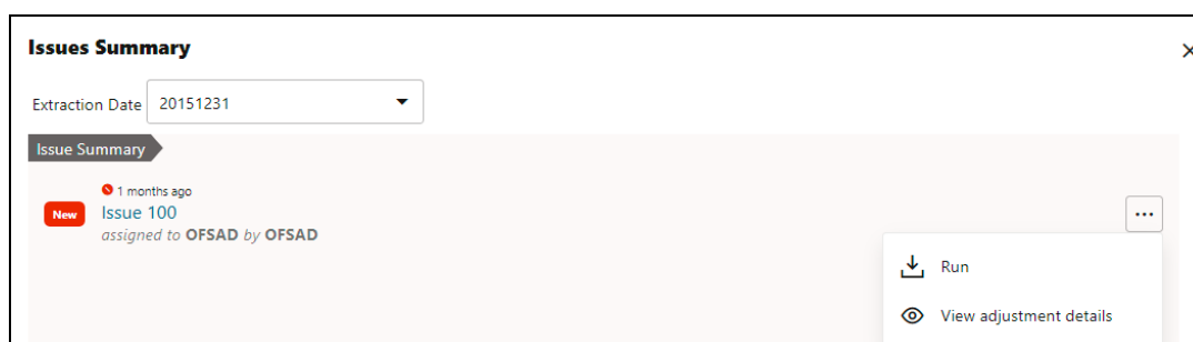
Figure 154: Issues Summary
