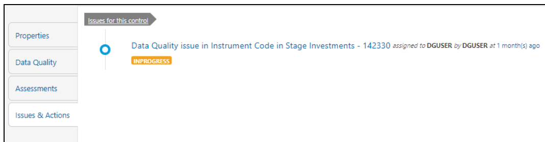
Figure 142: Issues & Actions
