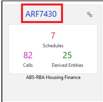
Figure 52: Report Information
