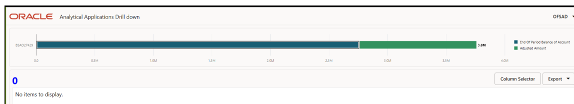
Figure 299: Measure Values
