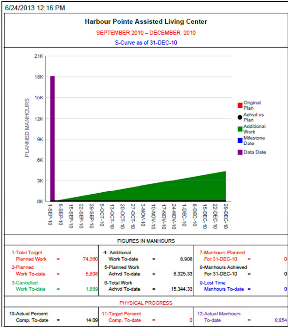
Figure 39: S 曲线
