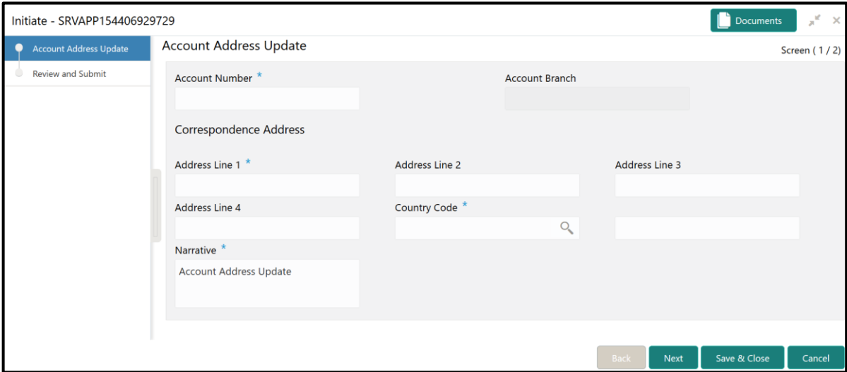
Figure 240: Account Address Update
