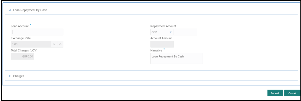
Figure 218: Loan Repayment By Cash (without Multi Currency and Total Charges)
