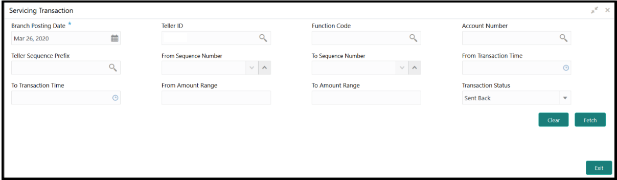
Figure 222: Servicing Transaction
