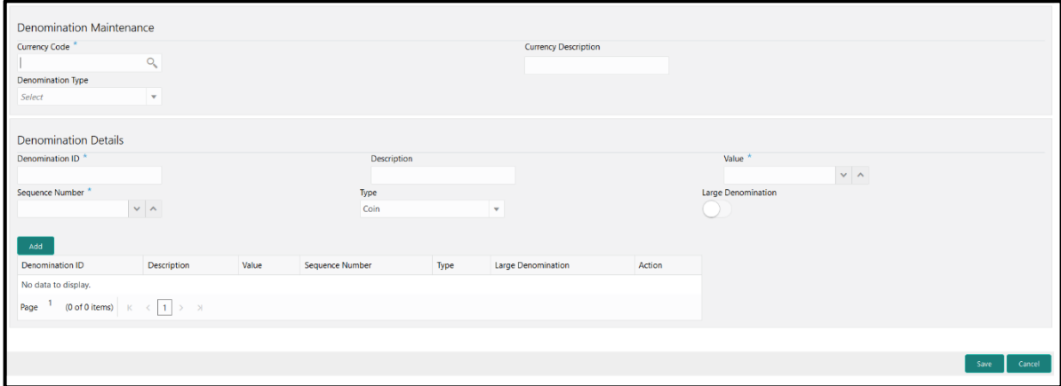
Figure 262: Denomination Maintenance
