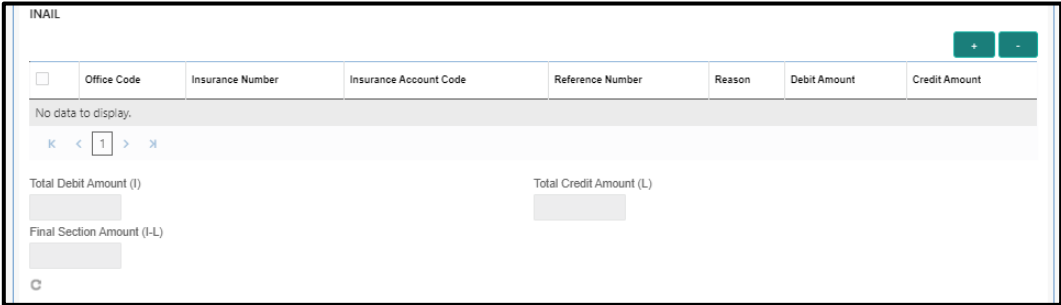
Figure 102: INAIL Details
