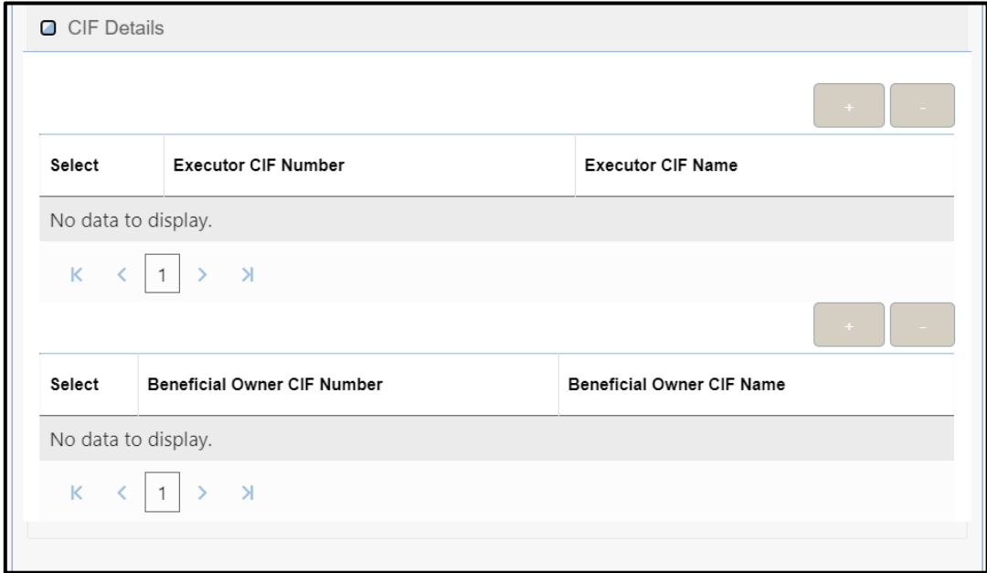
Figure 35: CIF Details
