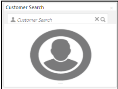
Figure 247: Customer Search
