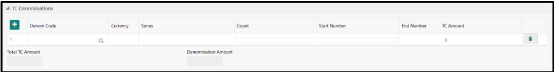
Figure 72: TC Denomination
