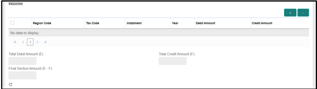
Figure 84: REGIONI Details
