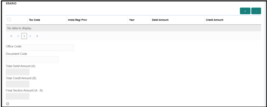
Figure 82: ERARIO Details
