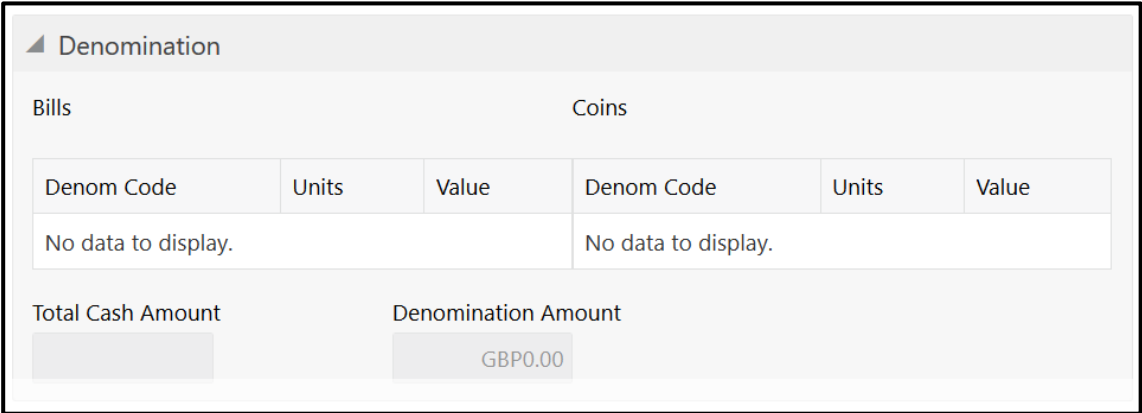
Figure 32: Denomination Details
