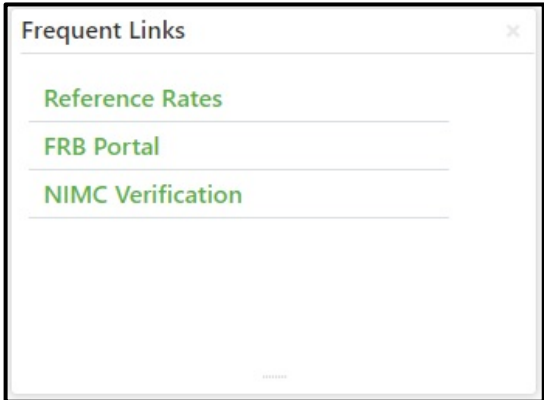
Figure 254: Frequent Links
