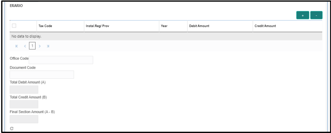
Figure 98: ERARIO Details
