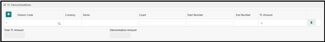
Figure 69: TC Denomination
