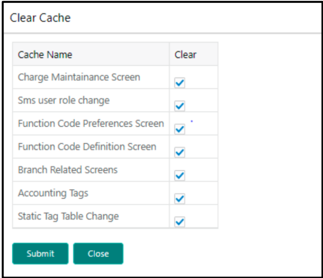
Figure 227: Clear Cache
