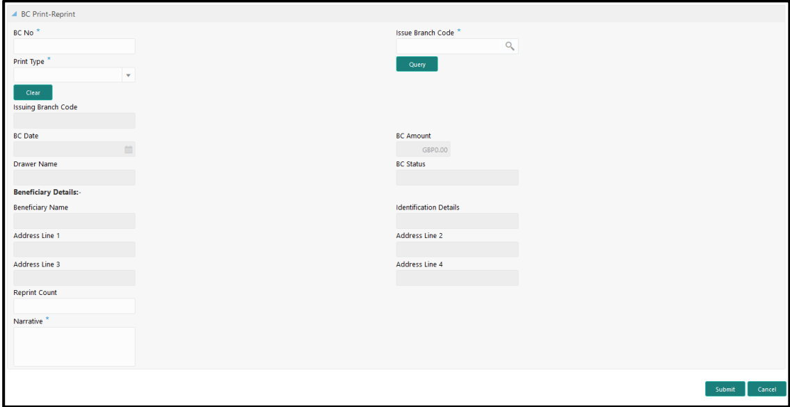
Figure 133: BC Print-Reprint
