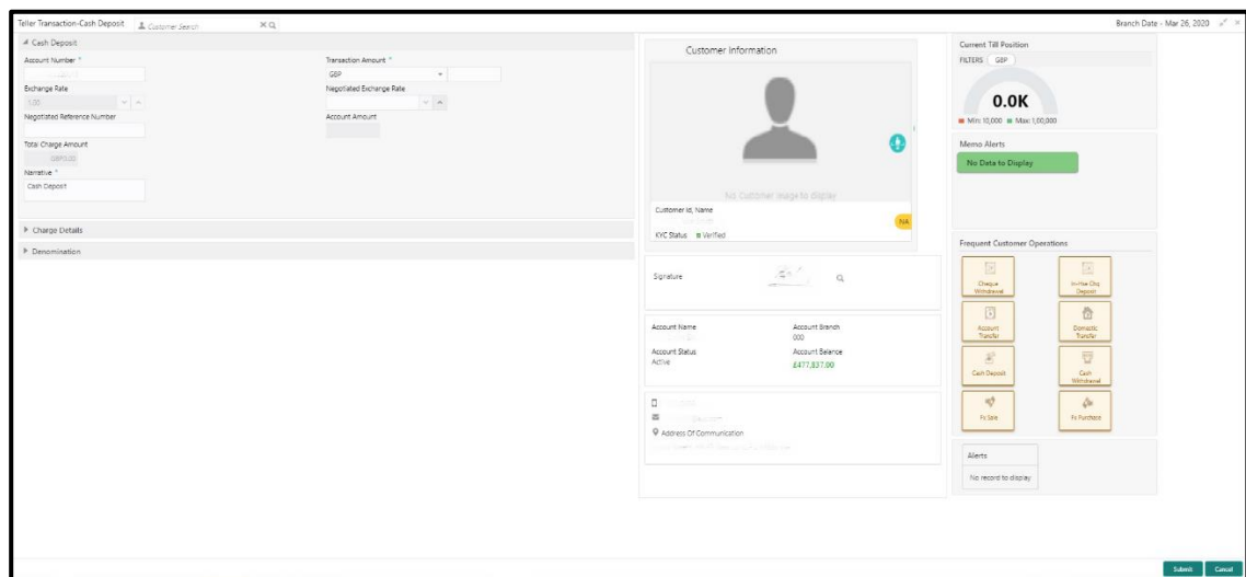
Figure 8: Transaction Area
