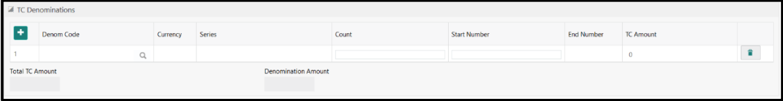
Figure 75: TC Denomination
