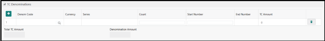
Figure 67: TC Denomination
