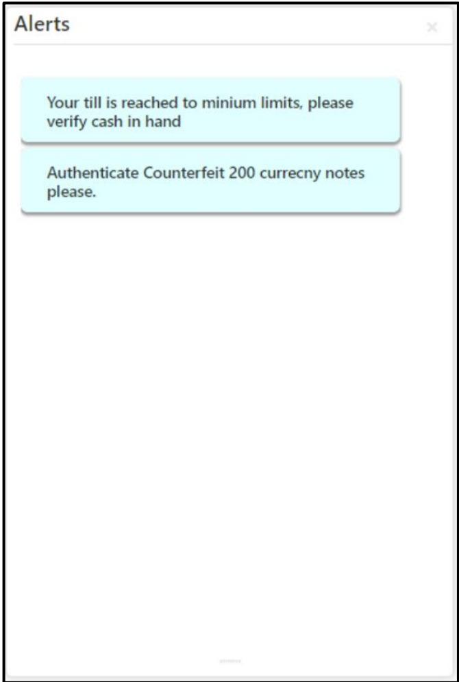
Figure 253: Alerts
