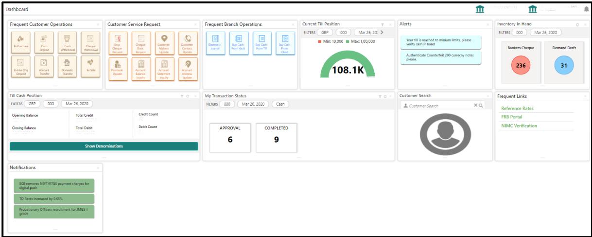
Figure 243: Branch Dashboard
