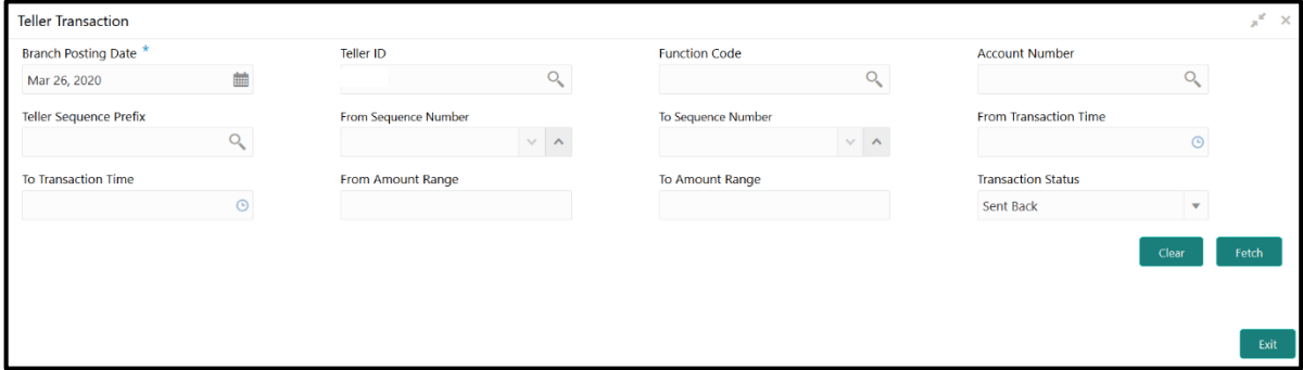
Figure 219: Teller Transaction
