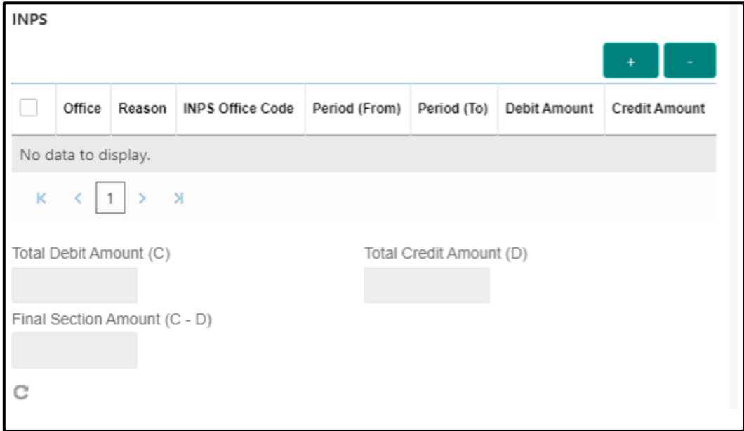
Figure 99: INPS Details
