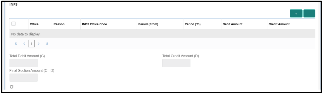
Figure 83: INPS Details
