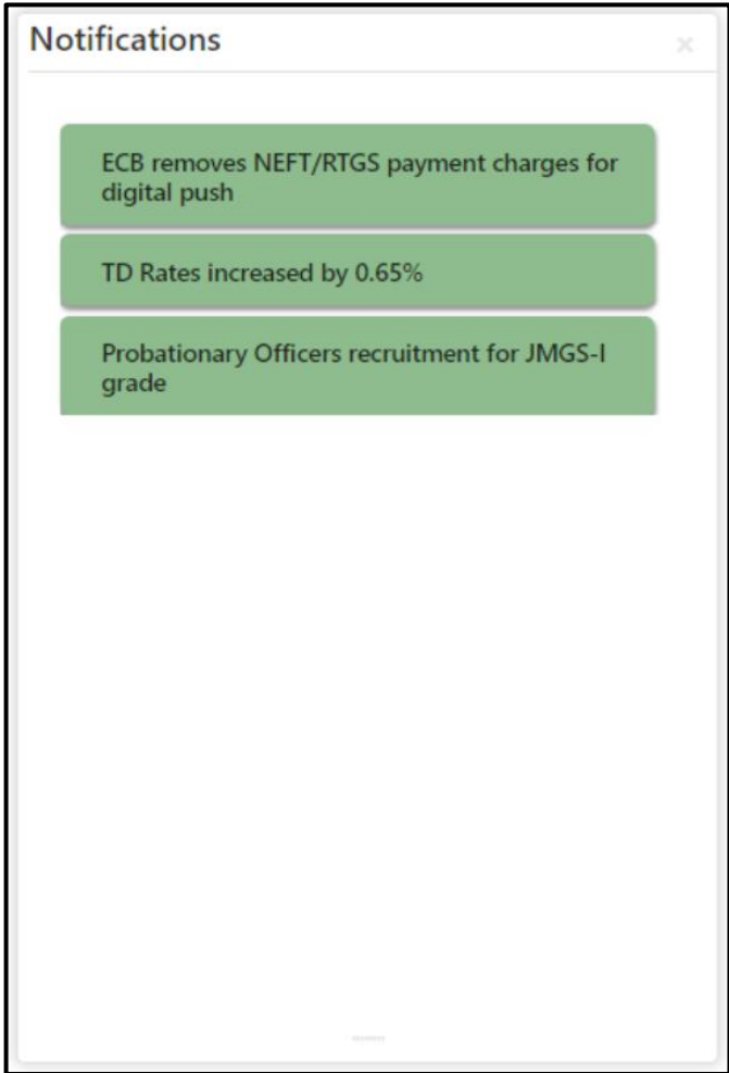
Figure 252: Notifications
