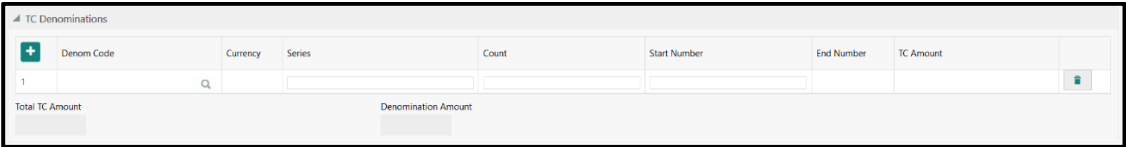
Figure 64: TC Denomination
