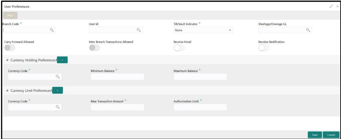
Figure 260: User Preference
