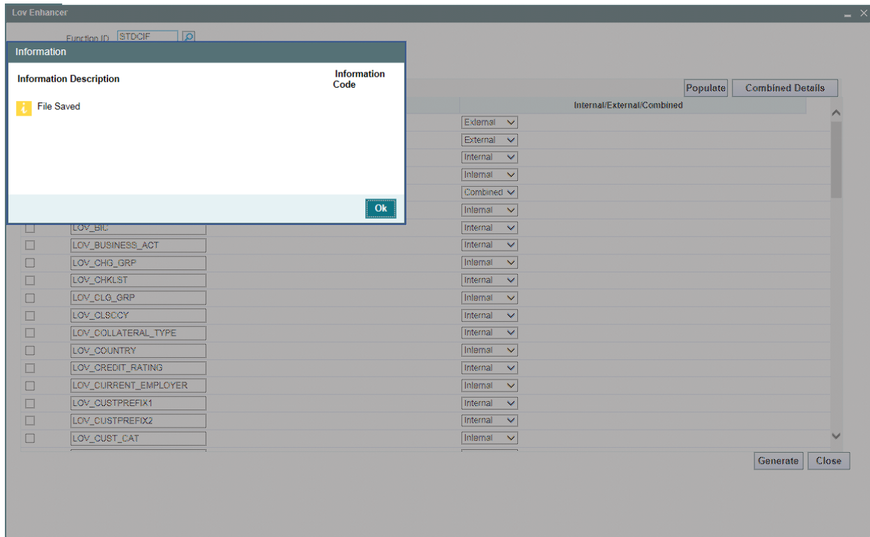
Fig 3.2.3: Generation Screen
