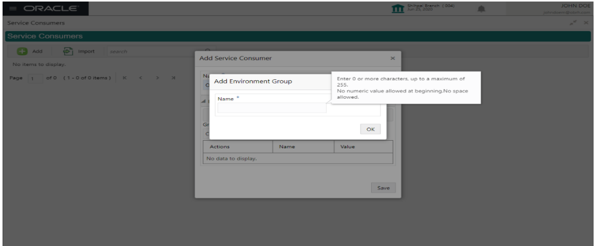
Figure 71: Environment Variables
