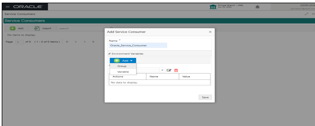
Figure 69: Environment Variables
