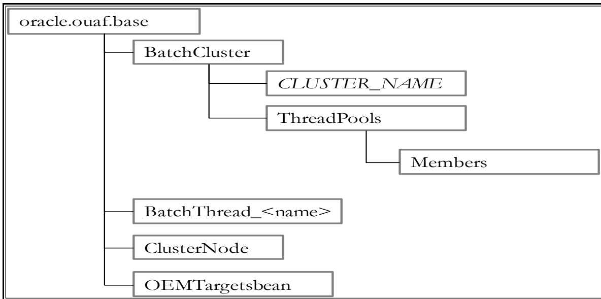
Figure 17: Batch Server Mbeans
