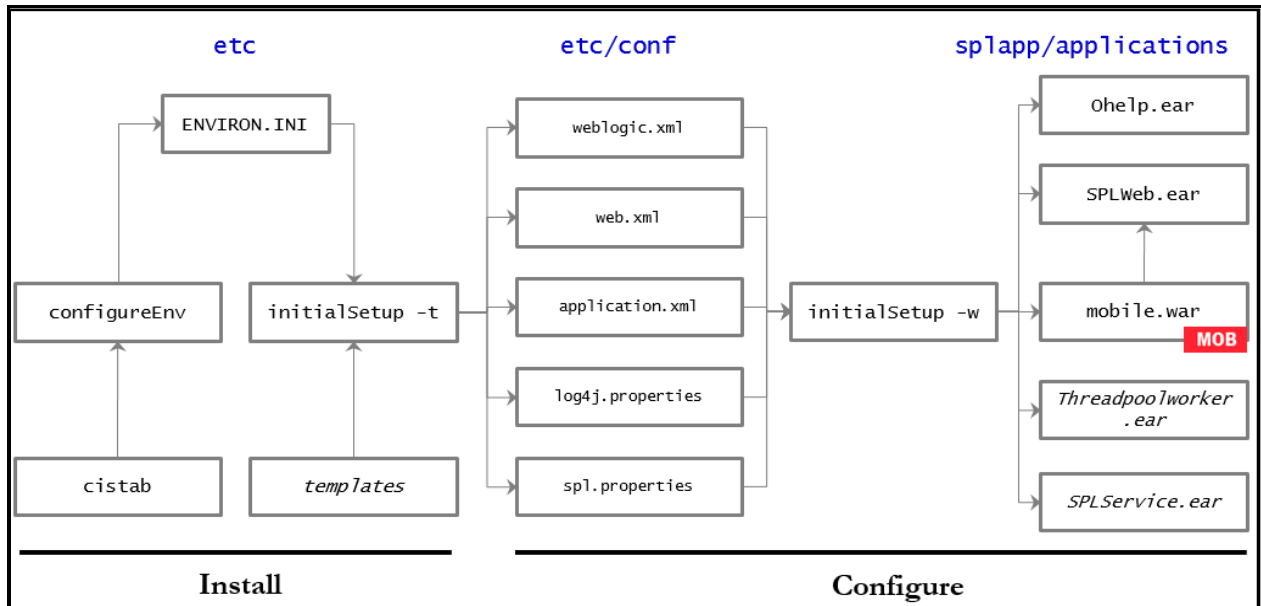
Figure 26: Web Application Server Configuration Process
