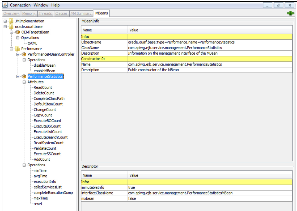
Figure 13: Business Application Server Mbeans in jconsole Example
