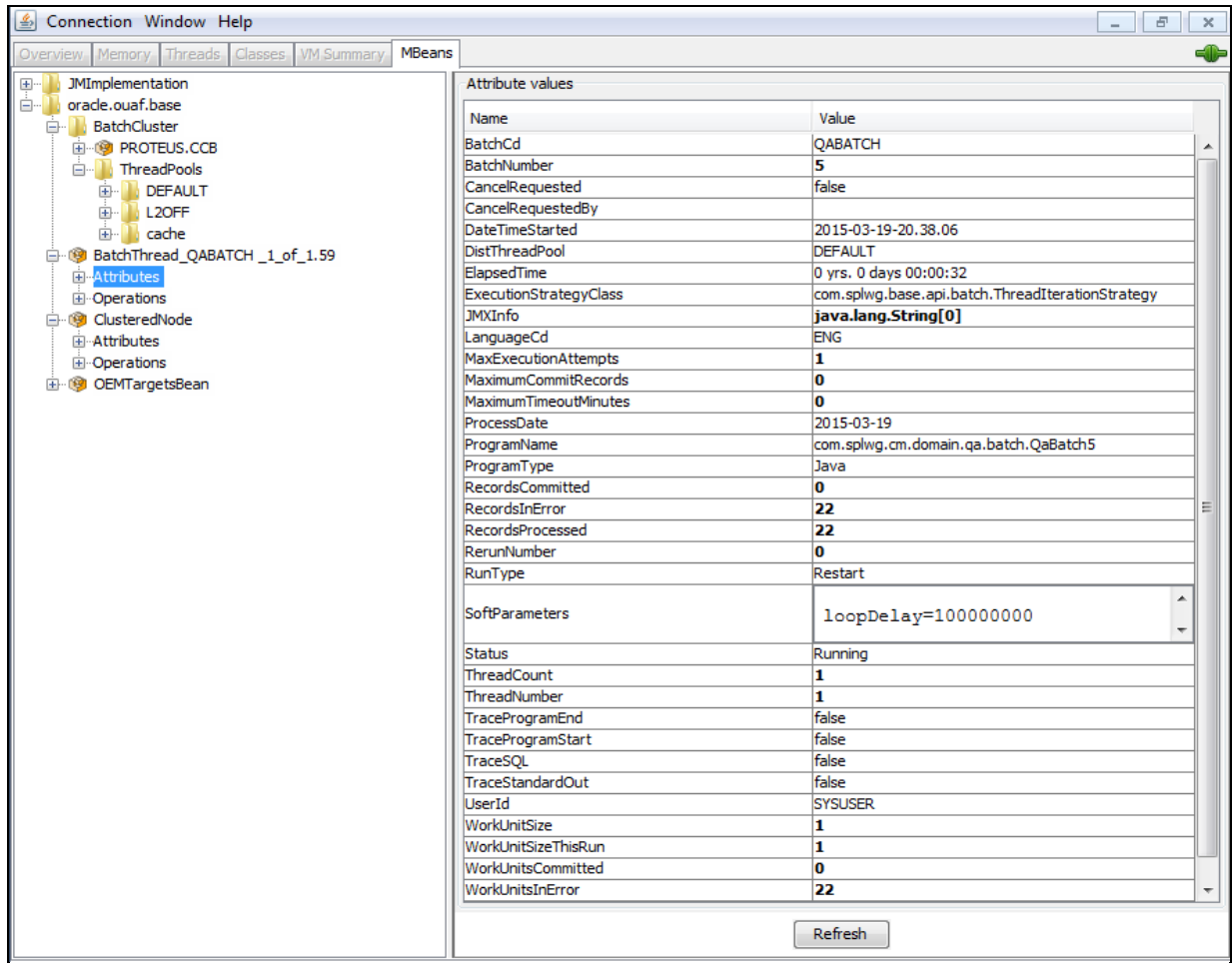
Figure 16: Batch Thread Mbean in jconsole Example
