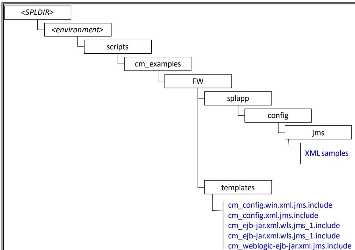
Figure 45: Custom JMS Configuration
