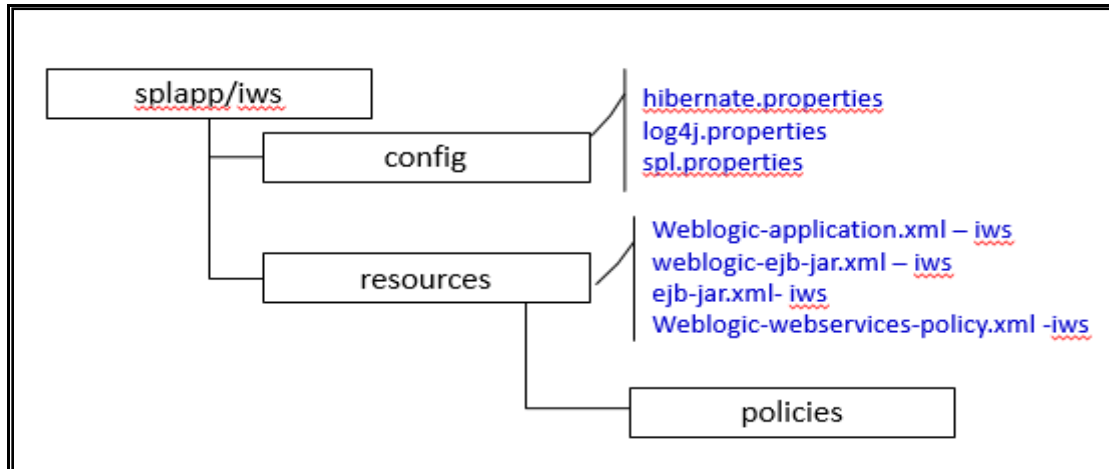
Figure 32 : Inbound Web Services Configuration
