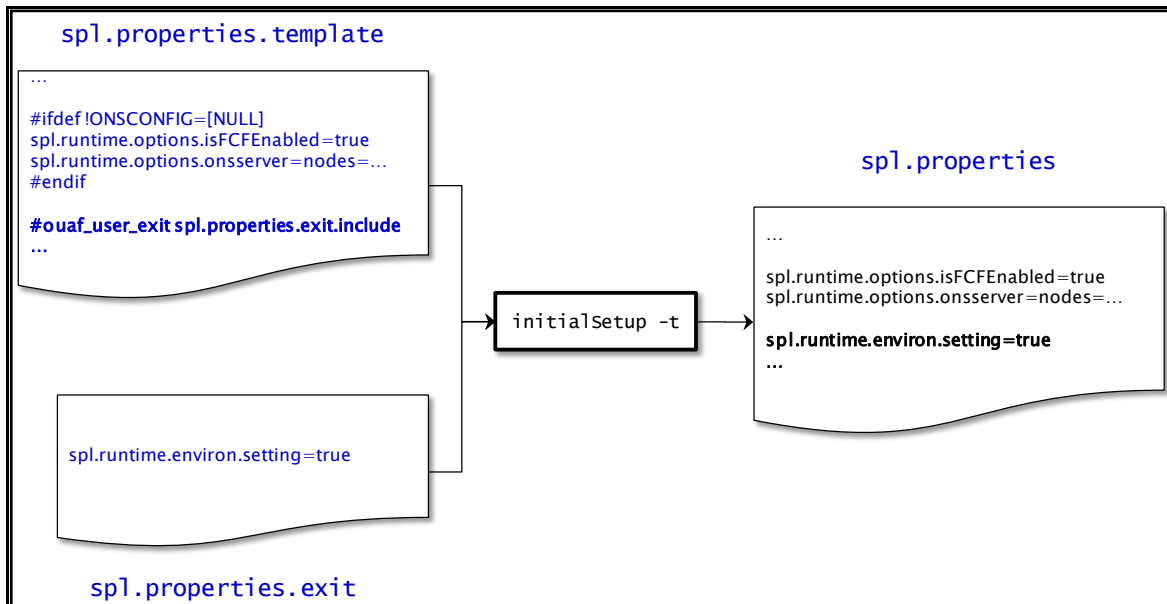
Figure 43: Include Files
