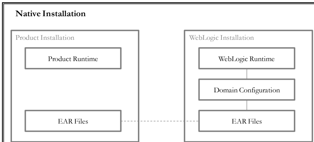
Figure 3: Native Architectures
