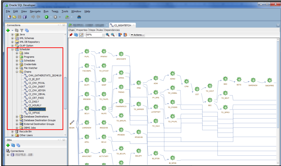
Figure 53: Example Oracle SQL Developer Oracle Scheduler Interface
