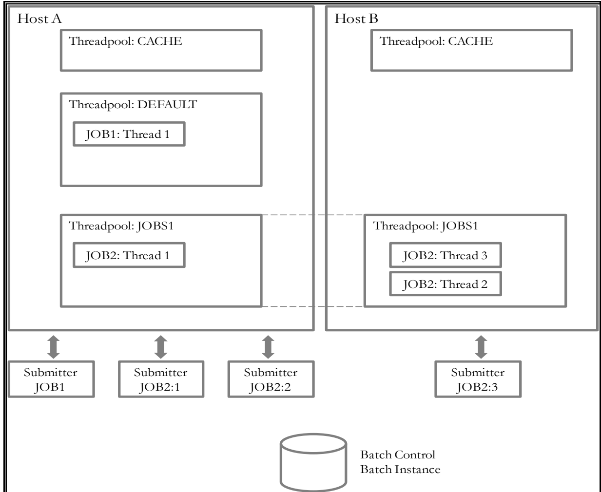
Figure 2: Batch Architecture Overview
