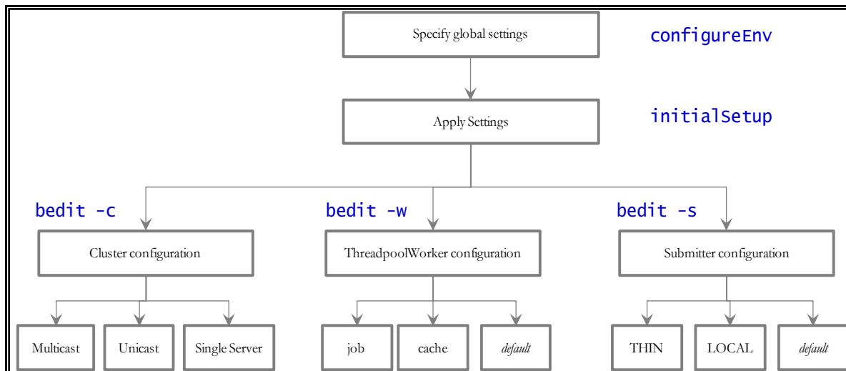
Figure 39: bedit Configuration Process
