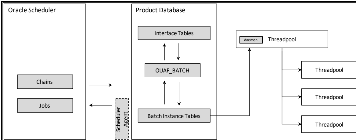
Figure 52: Oracle Scheduler Interface
