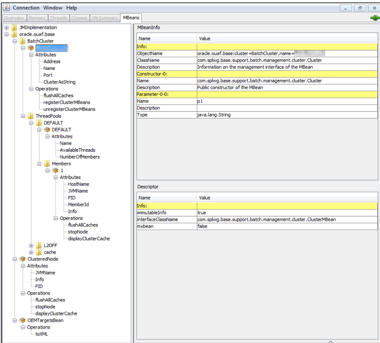
Figure 15: Batch Server Mbeans in jconsole Example
