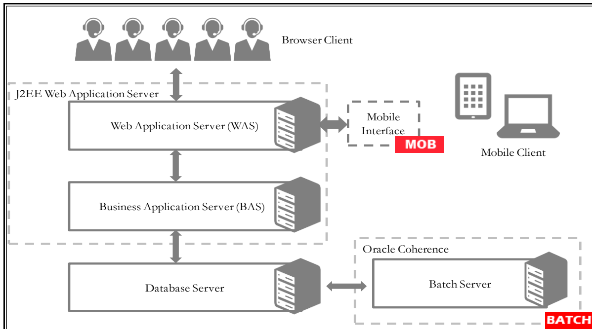
Figure 1: Product Architecture
