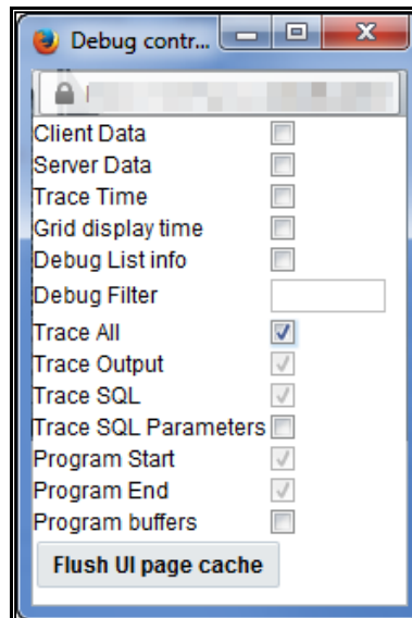
Figure 10: Debug Controls
