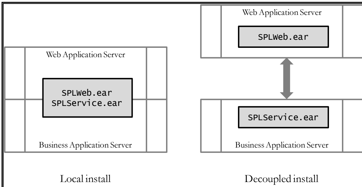
Figure 28: Installation Modes
