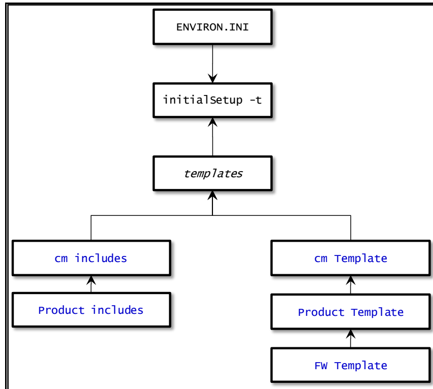
Figure 44: Template Hierarchy
