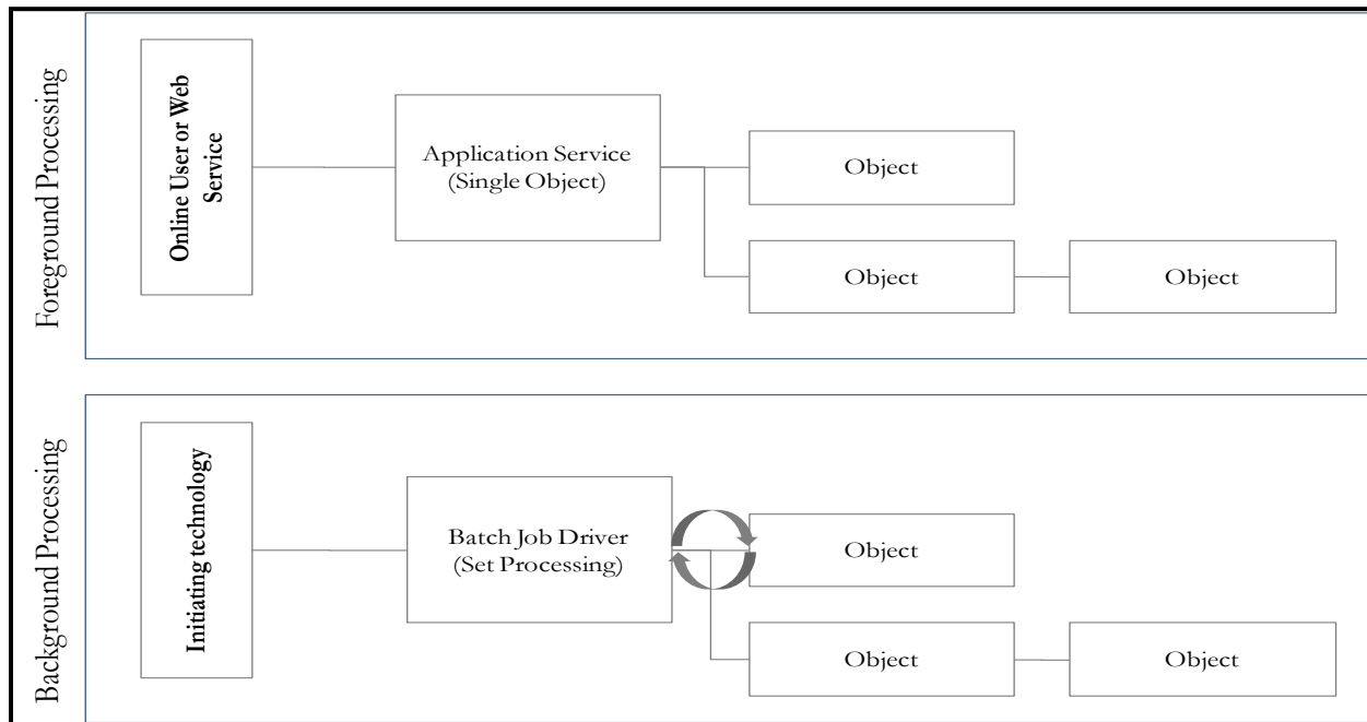
Figure 1: Batch Processing Architecture
