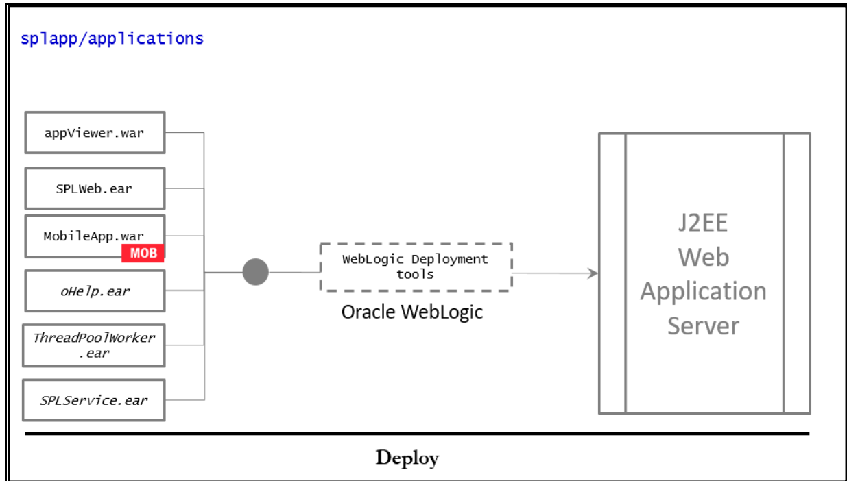
Figure 27: Web Application Server Deployment Process
