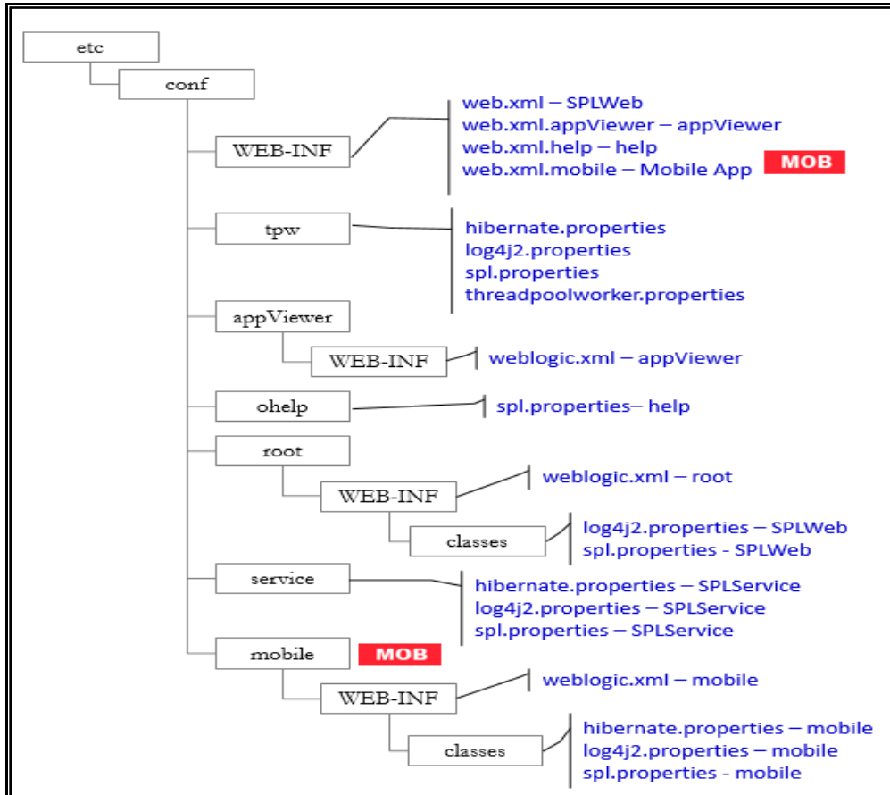
Figure 25: Configuration File Hierarchy
