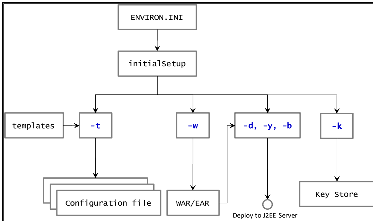
Figure 8: initialSetup Command Structure
