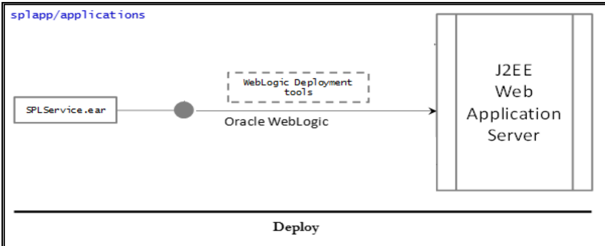
Figure 31 : Business Application Server Deployment Process
