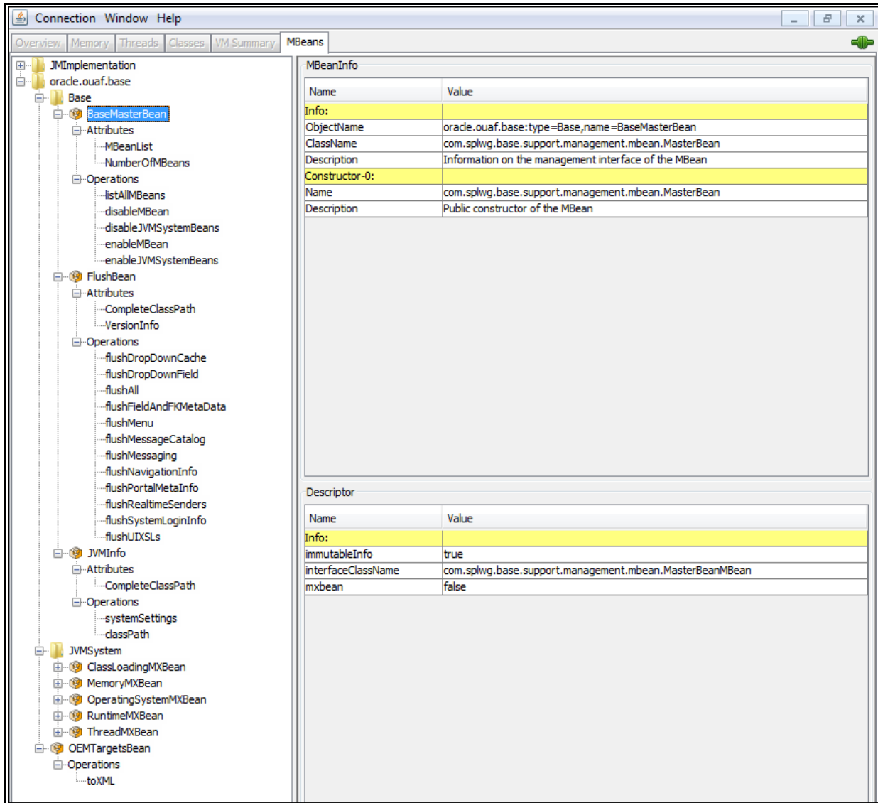
Figure 11: Example Web Application Server Mbeans in jconsole
