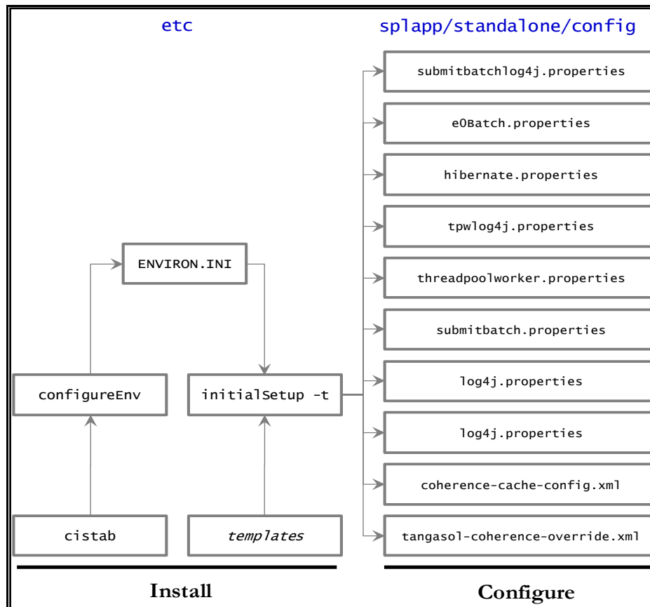
Figure 38: Batch Configuration Process
