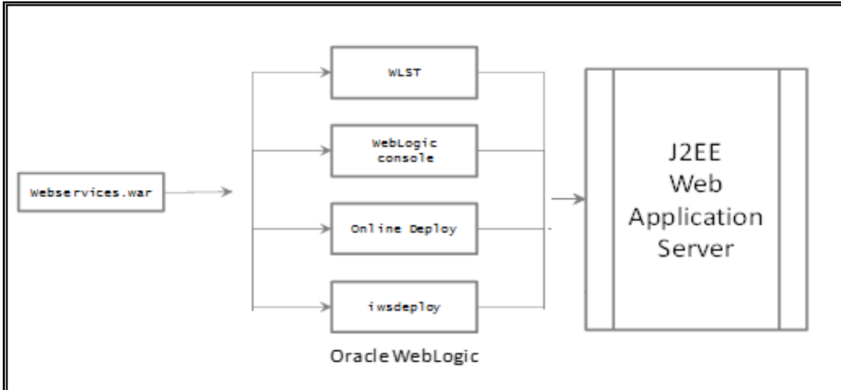
Figure 35: Inbound Web Services Deployment Process
