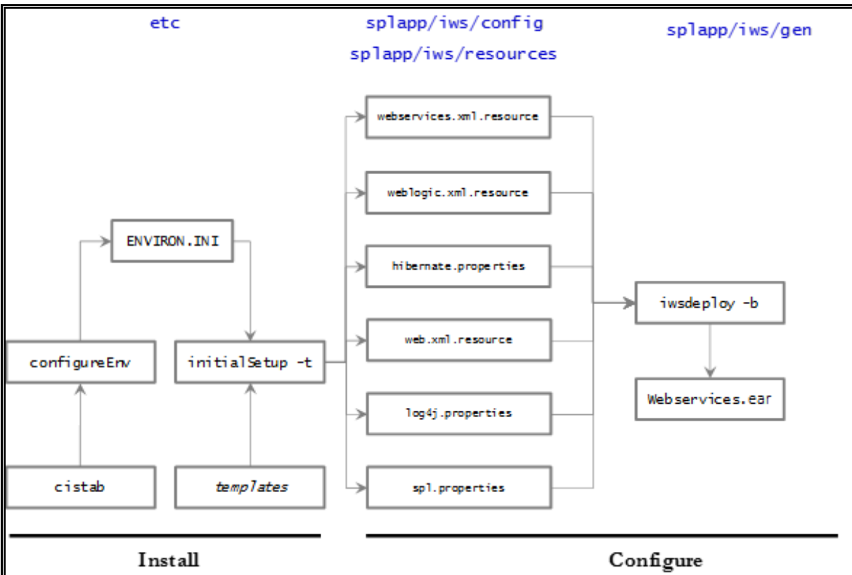
Figure 34: Inbound Web Services Configuration Process
