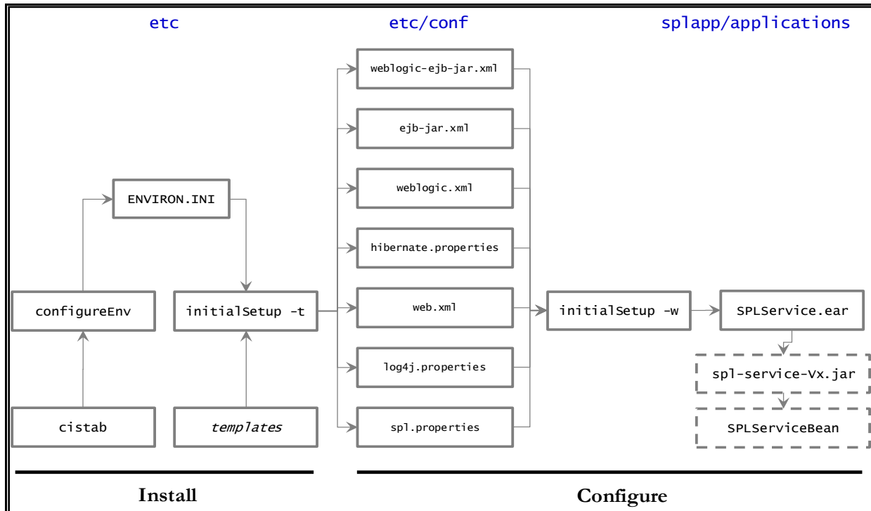
Figure 29: Business Application Server Configuration Process
