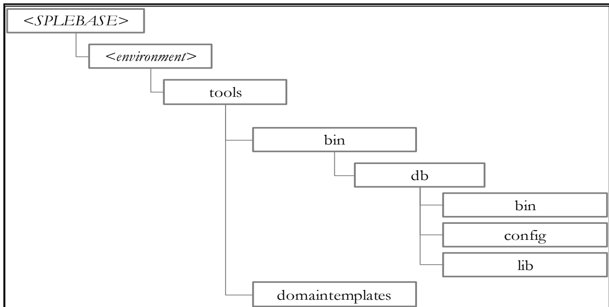
Figure 6: Tools Directory Structure
