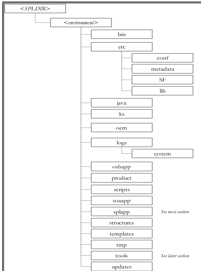
Figure 4: Software Directory Structure
