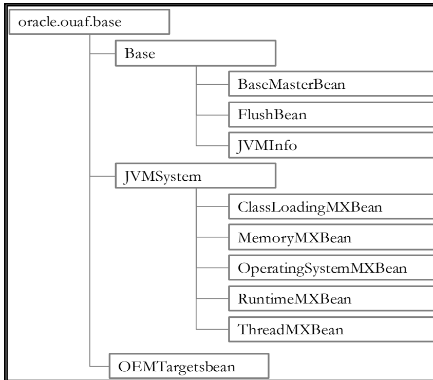
Figure 12: Web Application Server Mbeans
