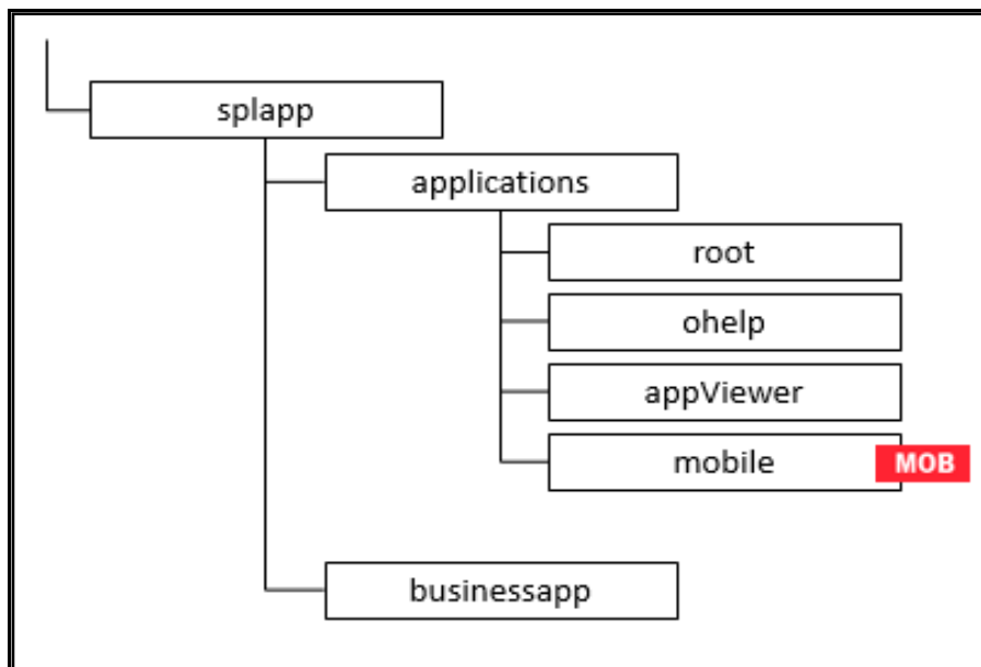
Figure 42 : Expanded Format
