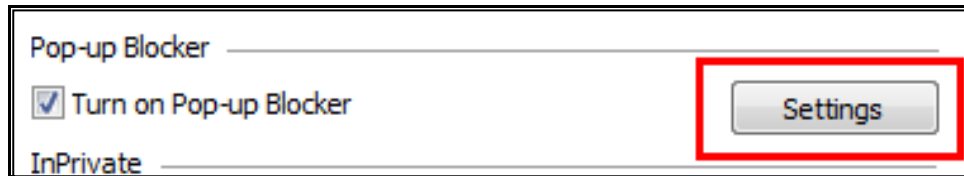
Figure 22 : Pop-up Blocker
