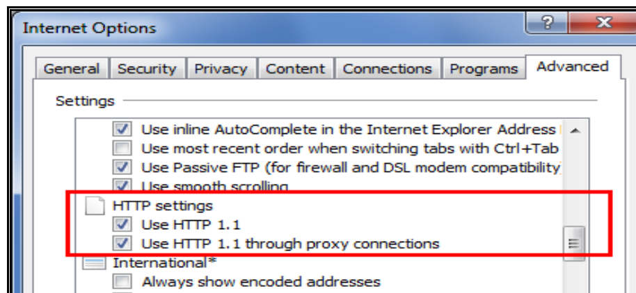
Figure 20 : HTTP 1.1 Settings
