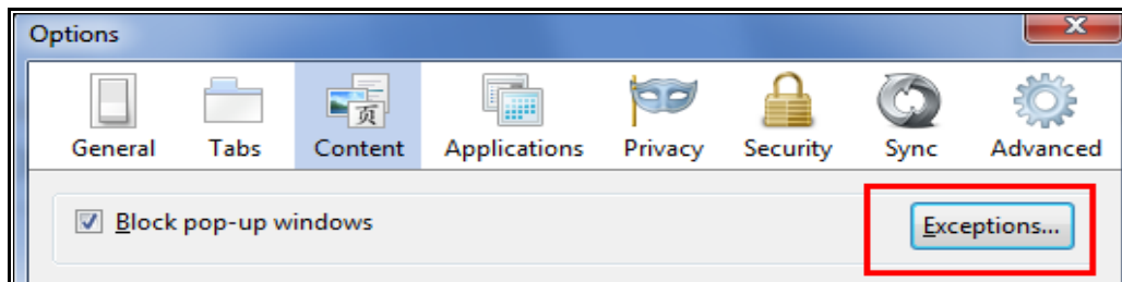
Figure 23 : Exceptions
