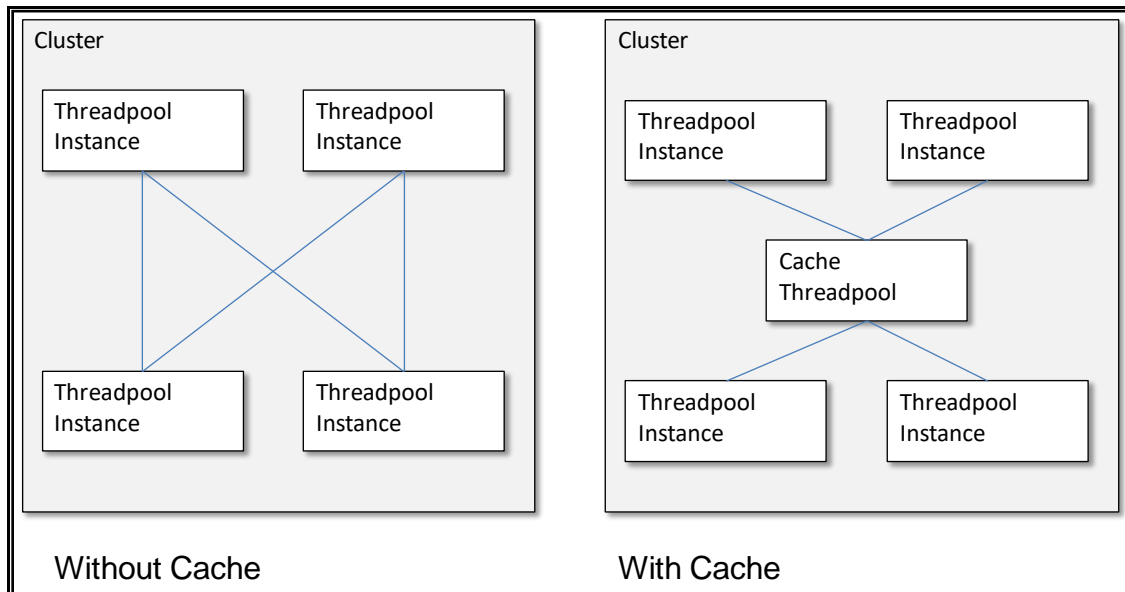
Figure 40 : Cache Architecture
