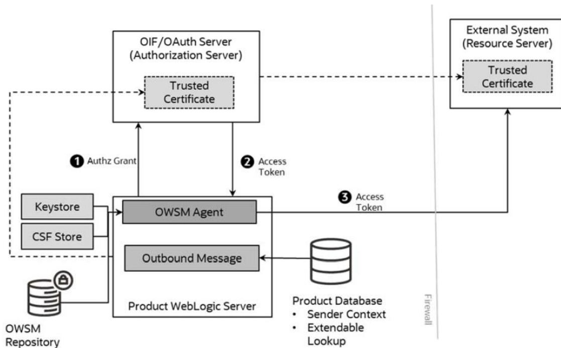
Figure 41: Federated Outbound Messages
