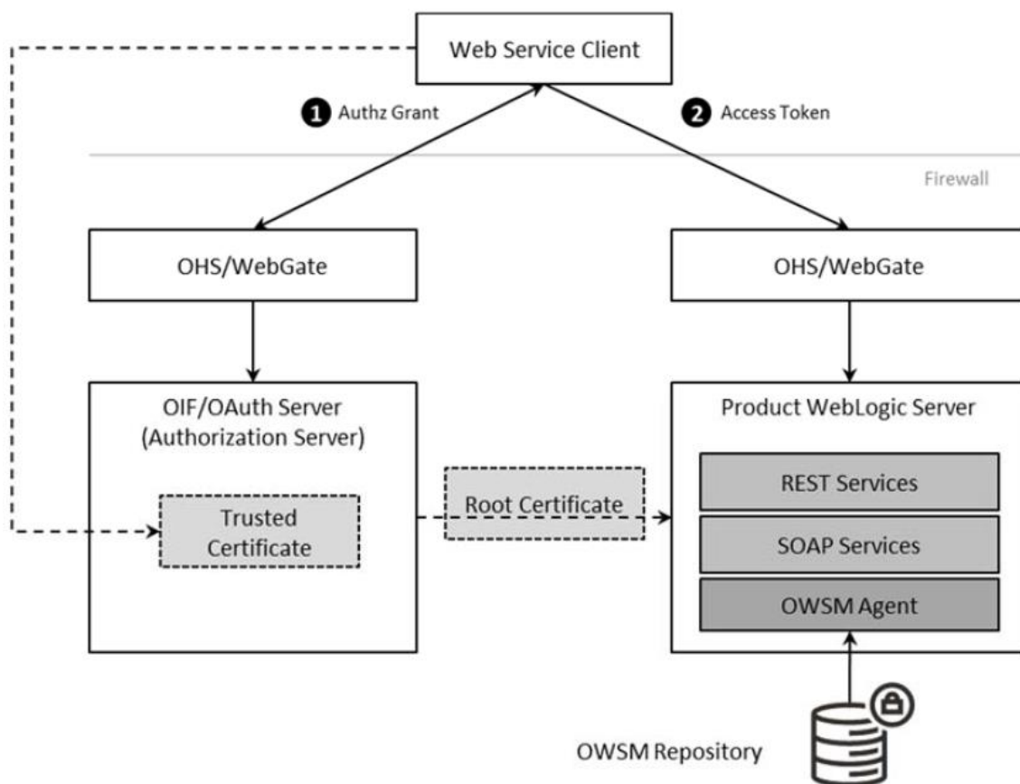
Figure 37: Federated Web Services Process Flow
