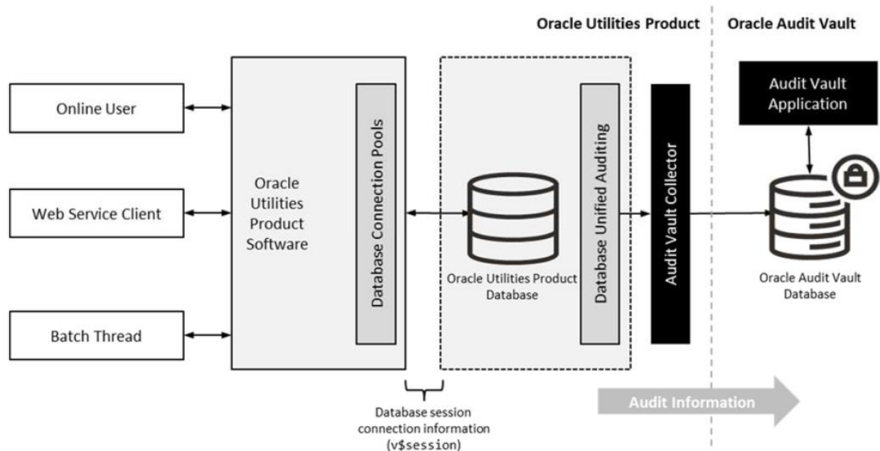
Figure 30: Using Audit Vault
