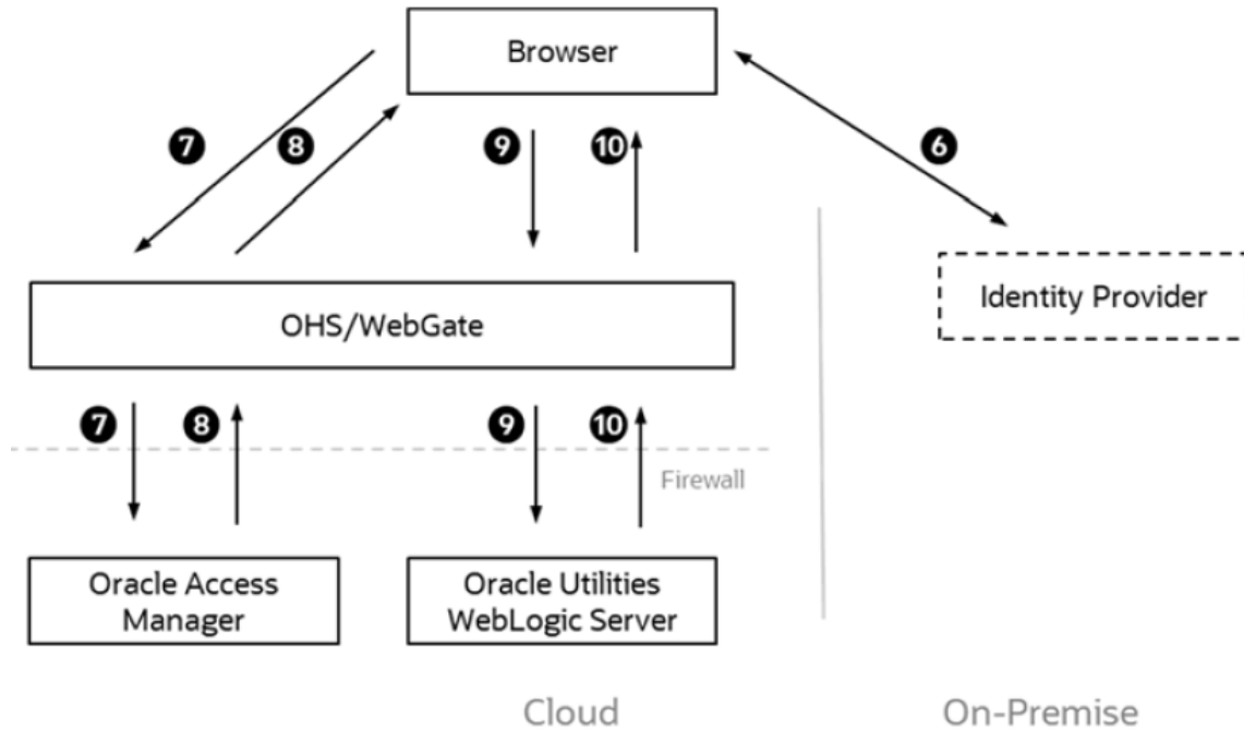
Figure 34: Federated Single Sign-On Process Flow – Part II
