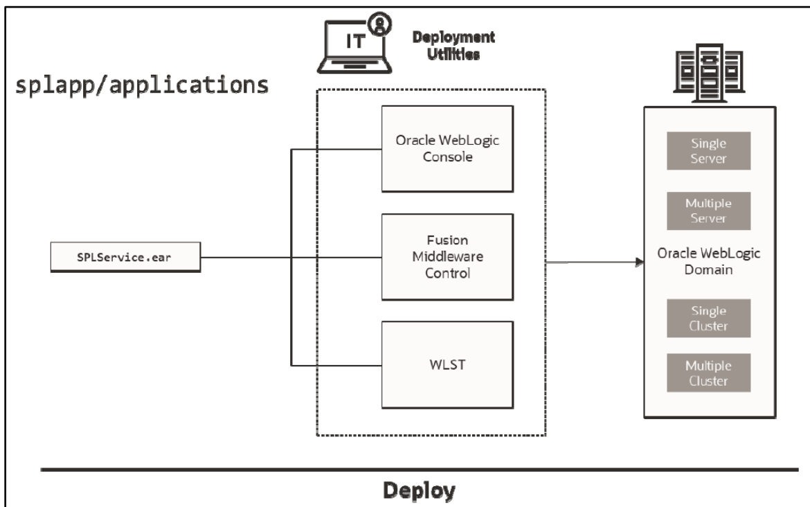
Figure 12 : Business Application Server Deployment Process
