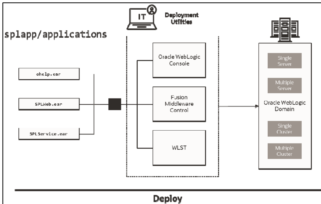
Figure 9: Web Application Server Deployment Process
