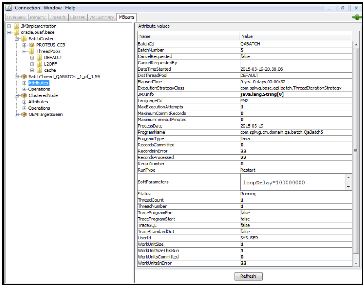
Figure 3: Batch Thread Mbean in jconsole Example
