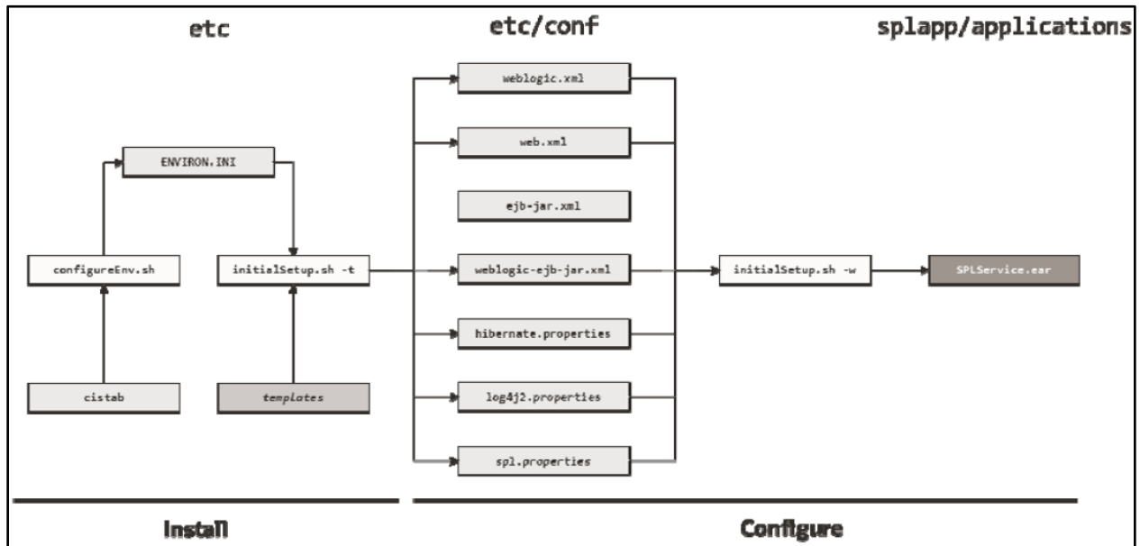
Figure 10: Business Application Server Configuration Process
