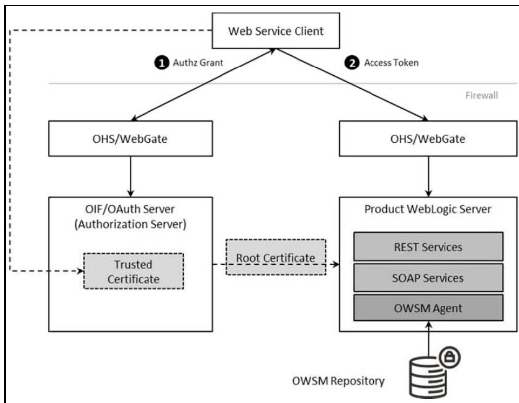
Figure 9: Federated Web Services Process Flow
