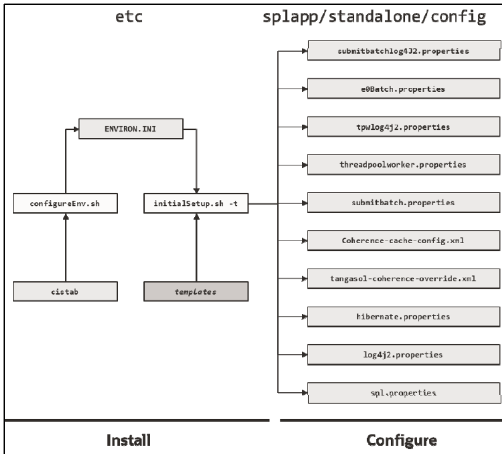
Figure 30: Batch Configuration Process
