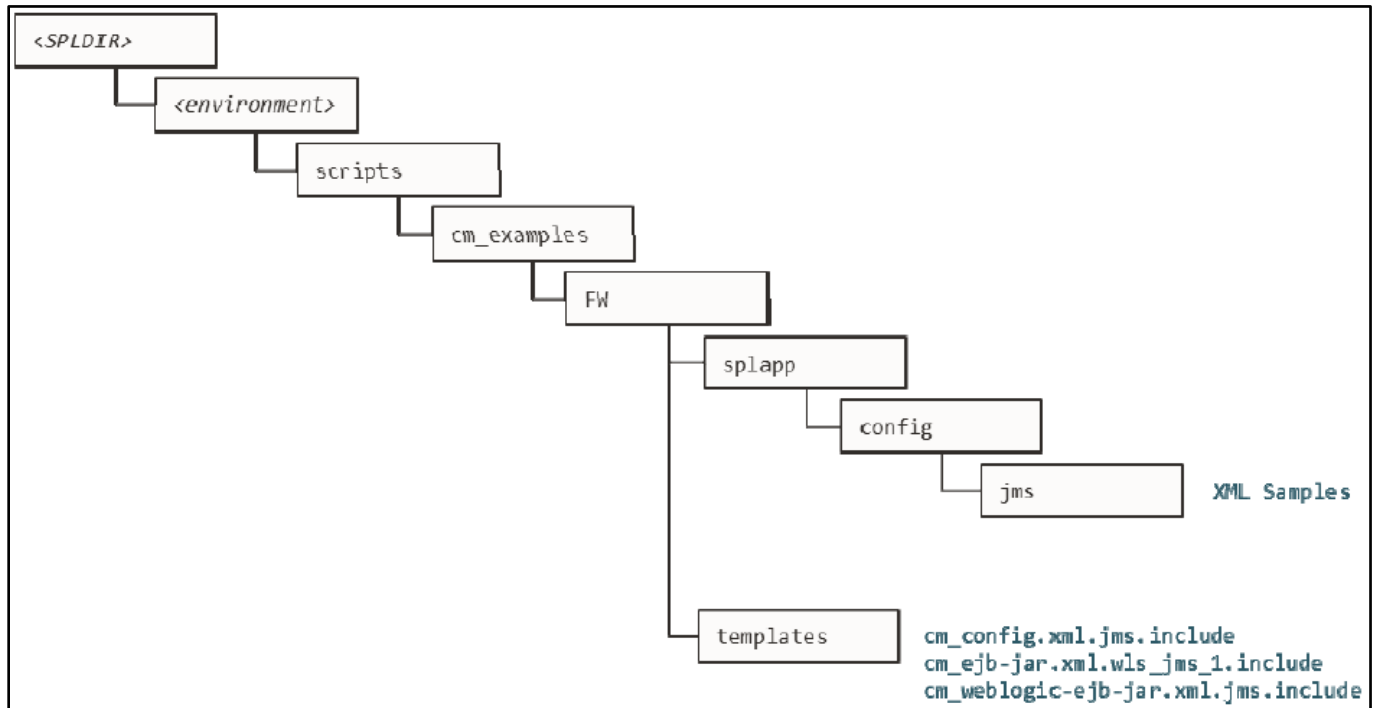
Figure 37: Custom JMS Configuration
