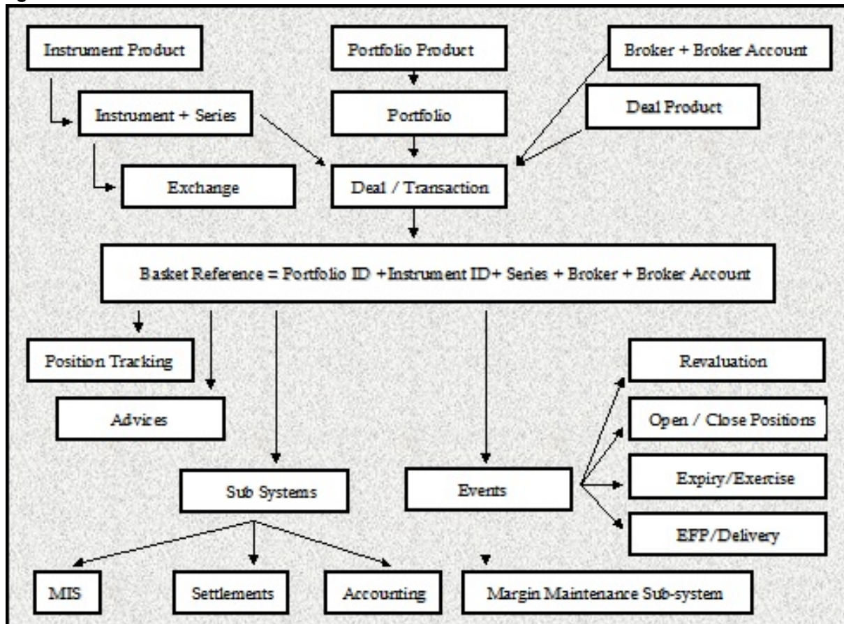
Figure 2.1: ETD Work-flow
