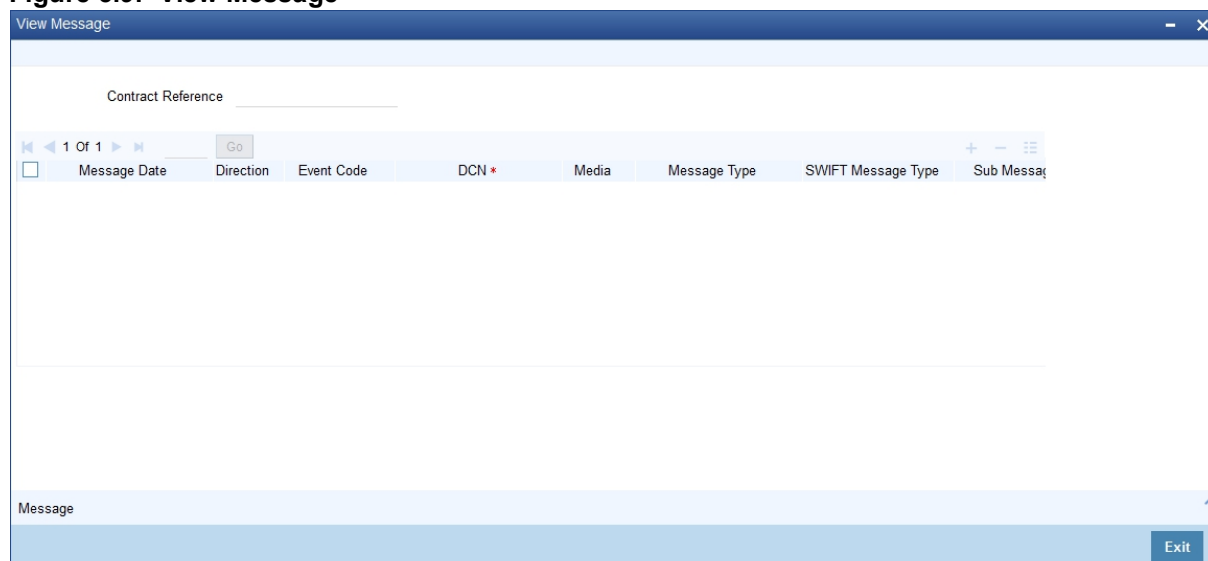
Figure 5.9: View Message
