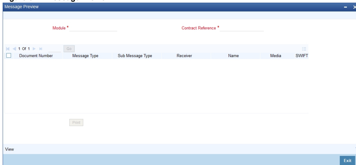
Figure 5.7: Message Preview
