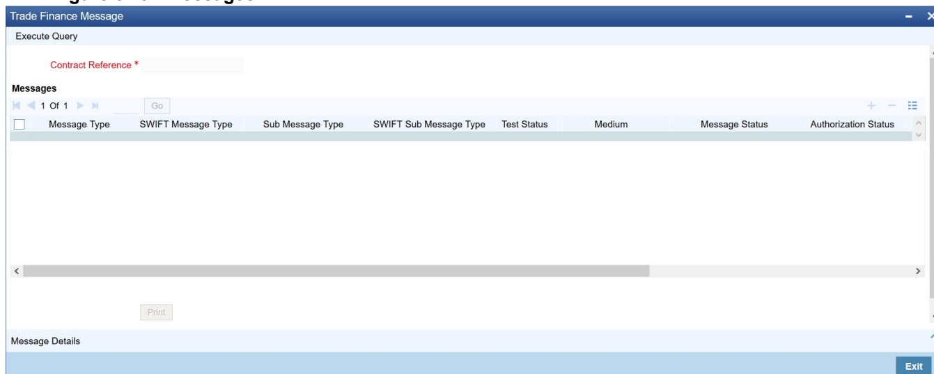
Figure 5.19: Messages
