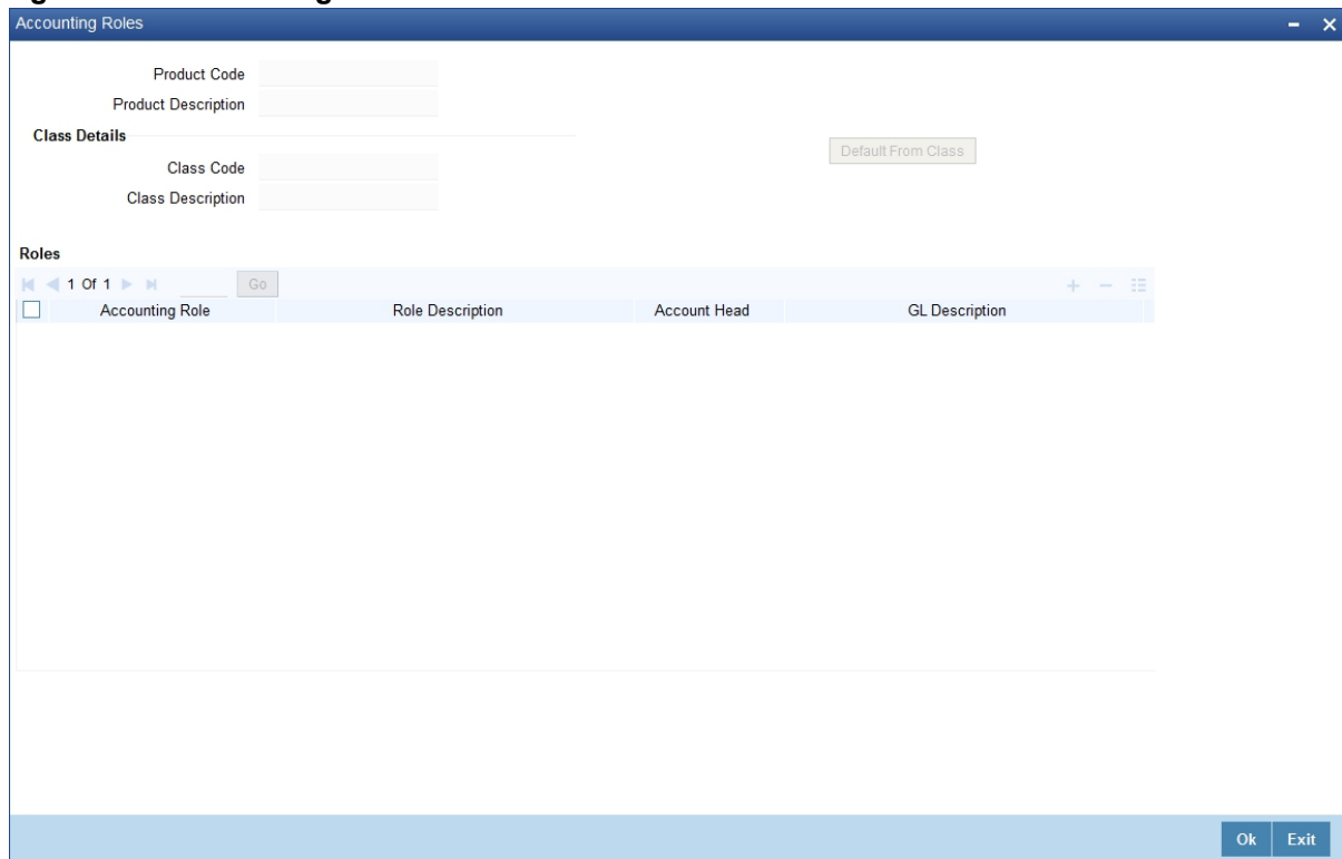
Figure 4.2: Accounting Roles
