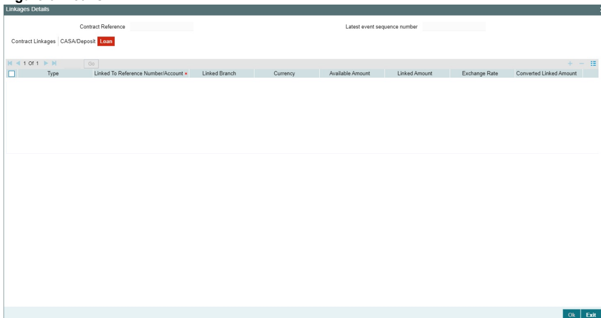
Figure 6: Loans
