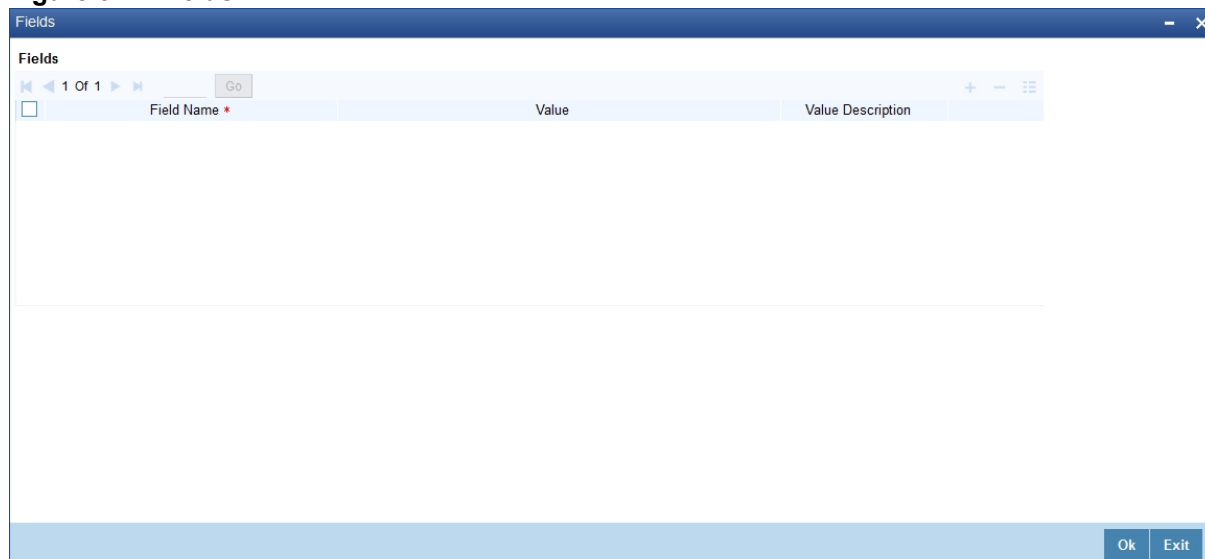
Figure 5.2: Fields
