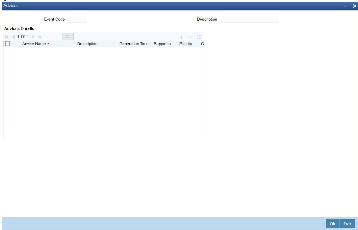
Figure 4.13: Advices
