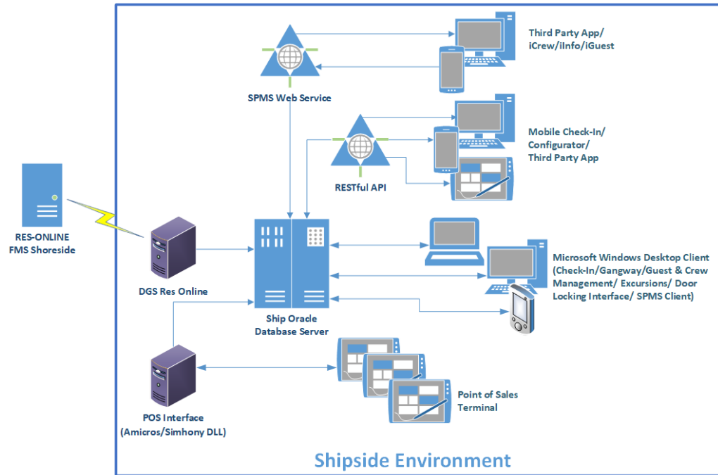
Figure 2-1 SPMS Network Architecture Diagram
