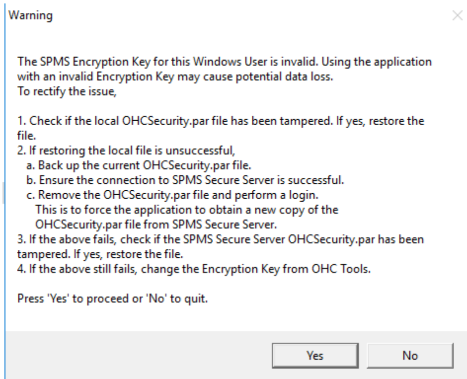
Figure 6-11 Invalid SPMS Encryption Key Warning
