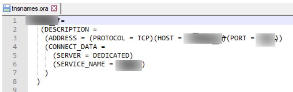
Figure 4-2 Sample TNS Configuration in Tnsnames.ora
