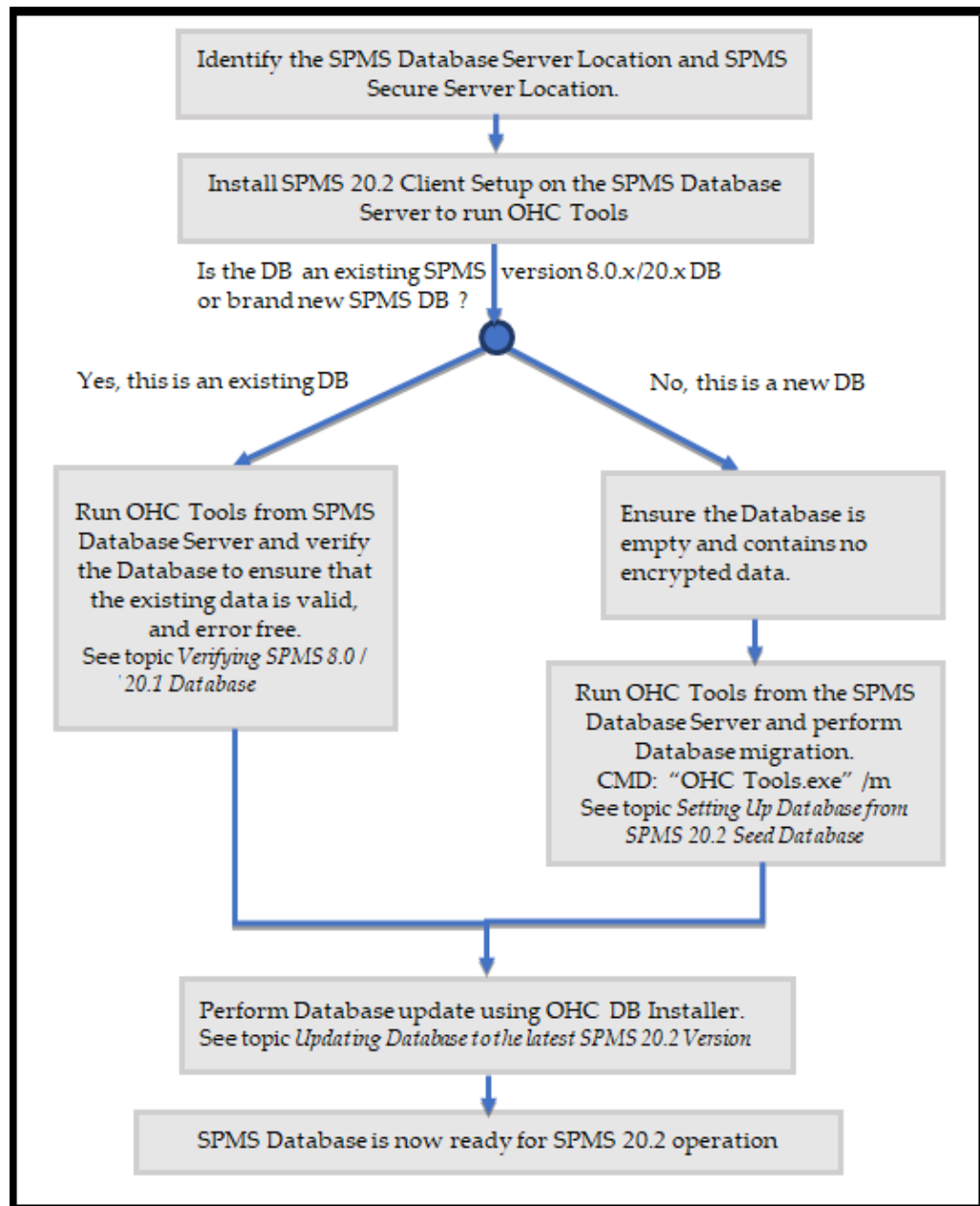
Figure 4-1 Database Preparation Workflow
