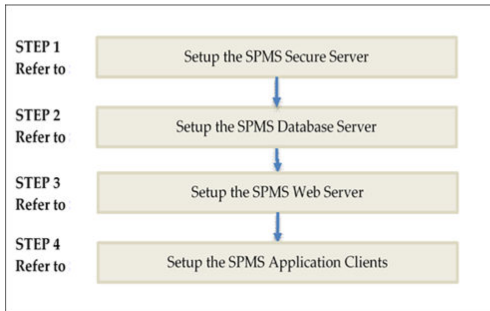
Figure 2-4 SPMS 8.0 Summarized Installation Process Flow
