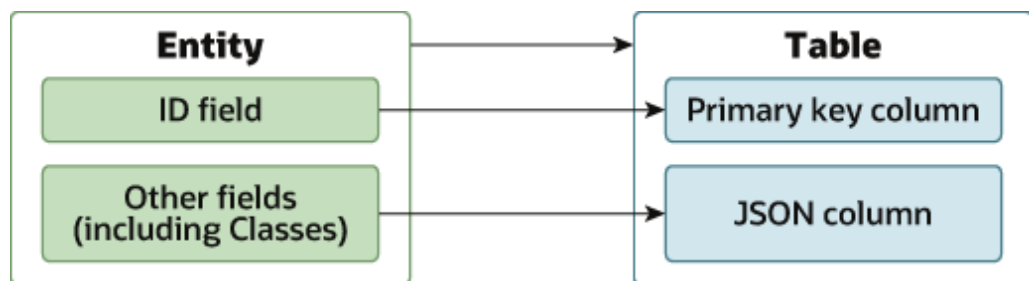
Figure 15-2 Persistence Model
