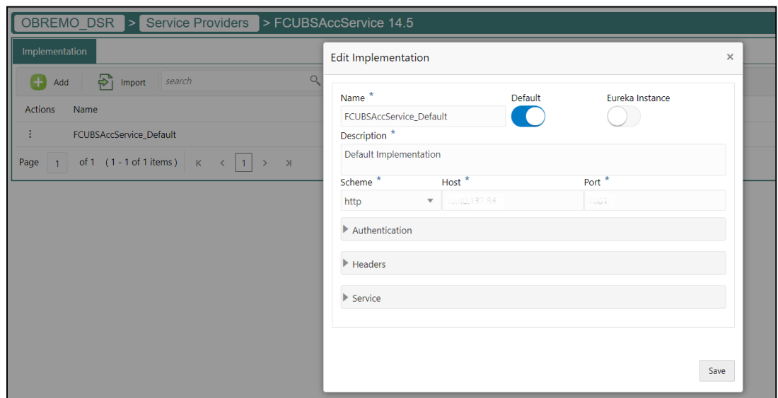
Figure 42: Edit Implementation
