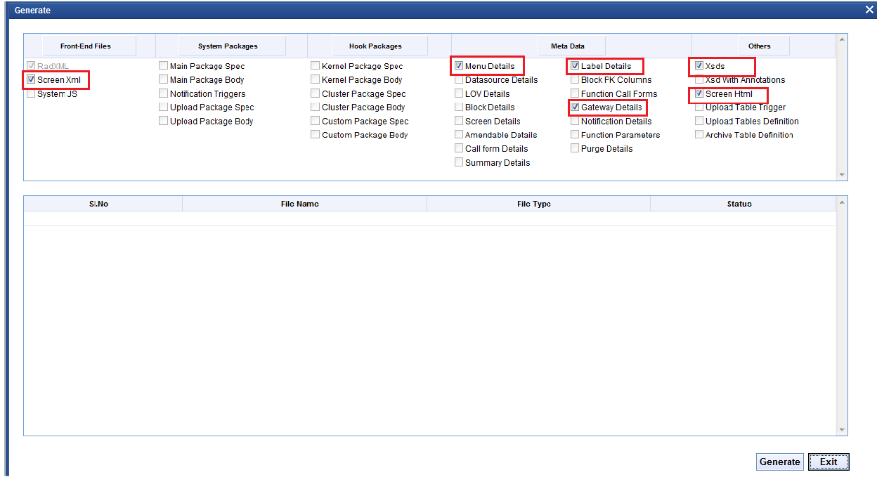
Fig 4.3: Generated Files
