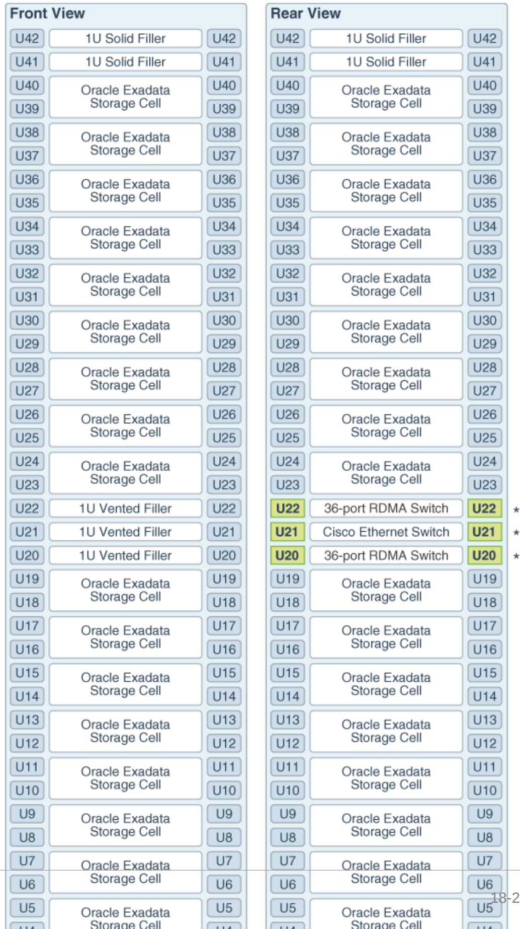
Figure 18-1 Rack Layout of Oracle Exadata Storage Expansion Full Rack X5 to X8M
