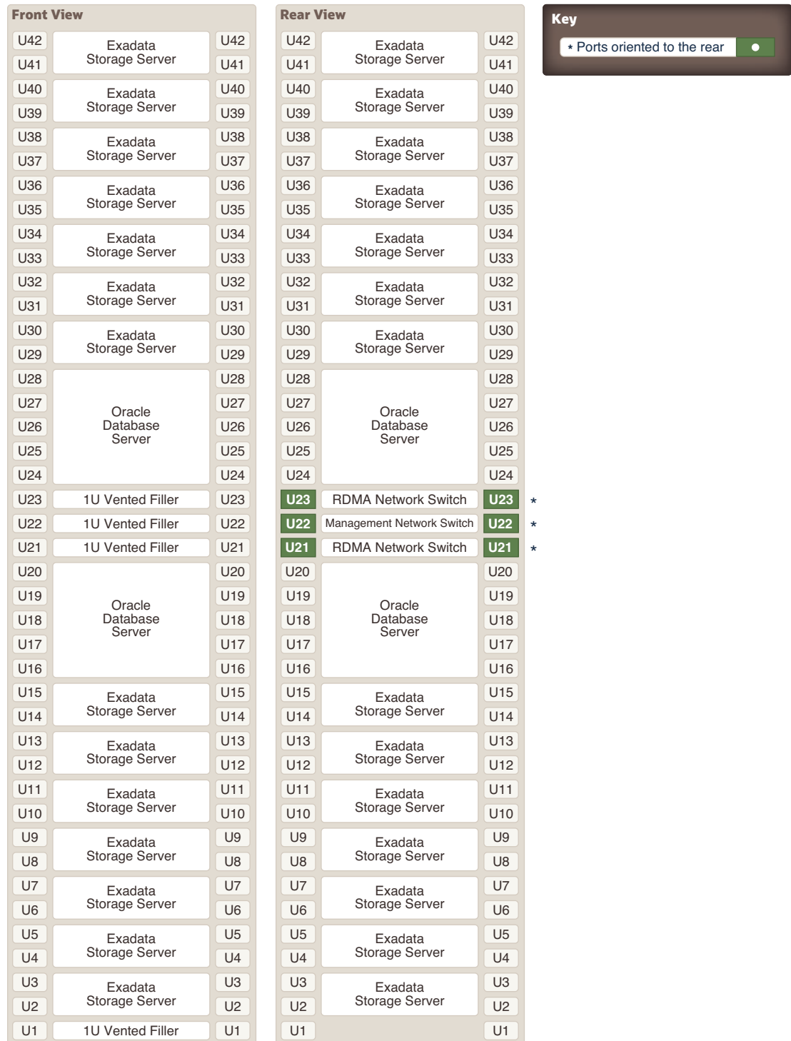
Figure 11-2 Rack Layout of Exadata Database Machine X8M-8
