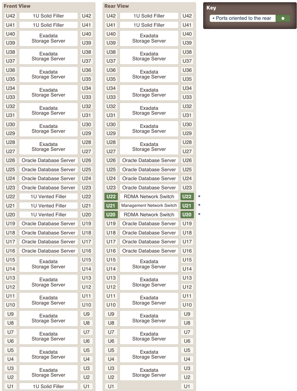
Figure 11-1 Rack Layout of Exadata Database Machine X8M-2 Full Rack
