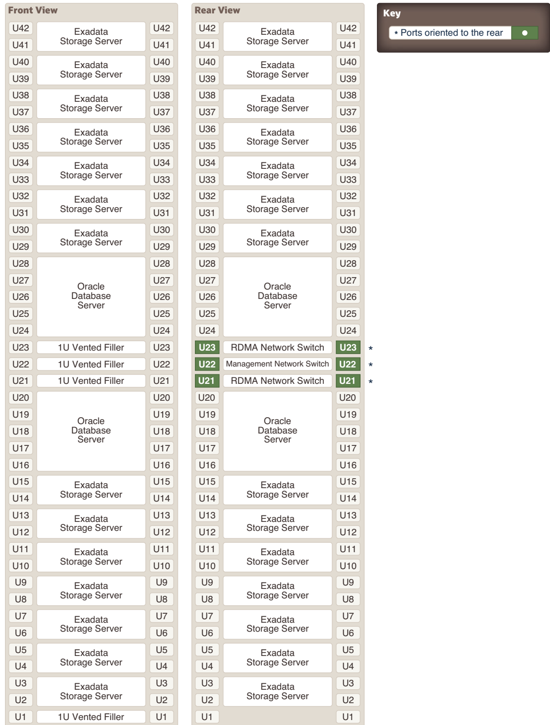
Figure 10-2 Rack Layout of Exadata Database Machine X9M-8
