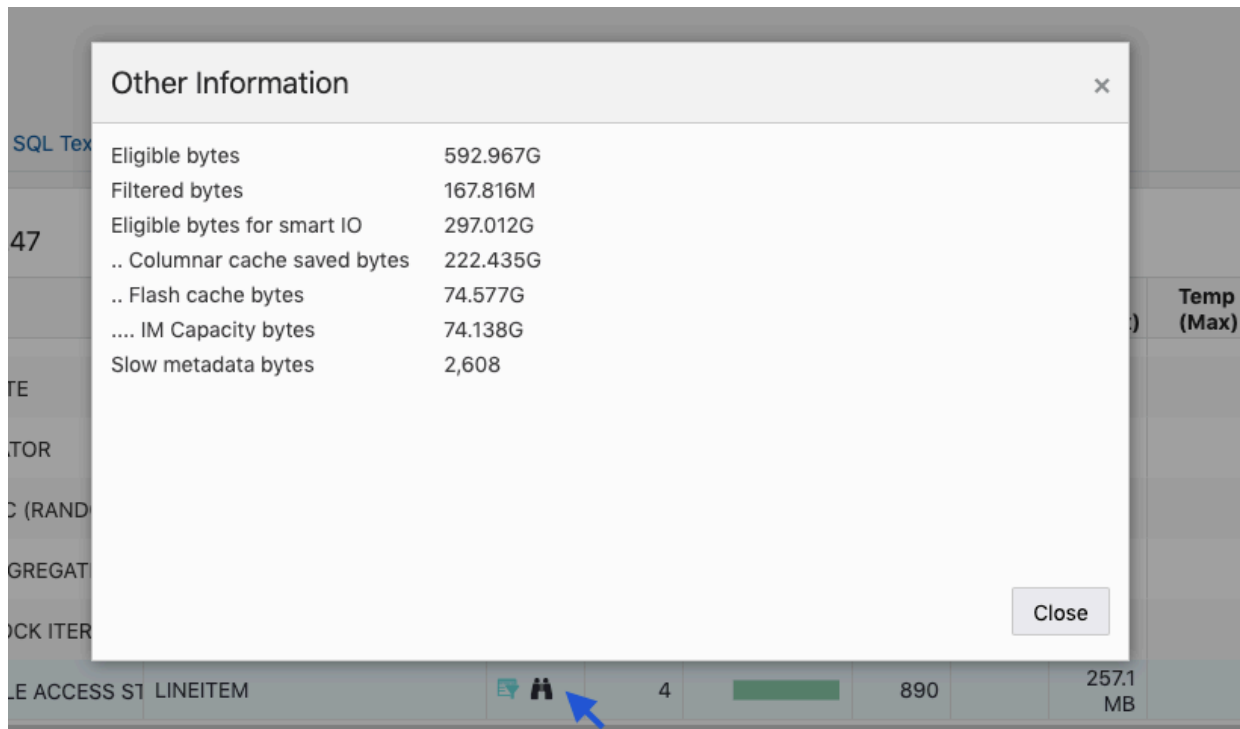
Figure 7-18 SQL Monitor Report: Smart I/O Row Source Statistics
