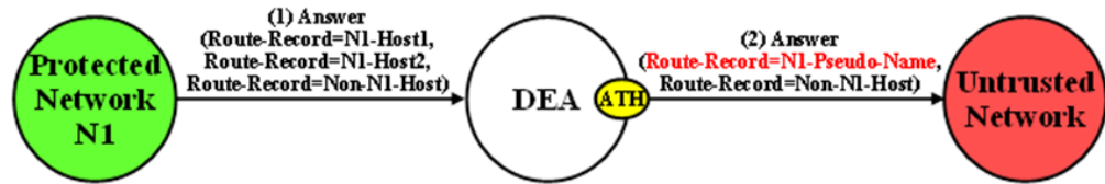
Figure 10-7 Route-Record Hiding - Answer Message
