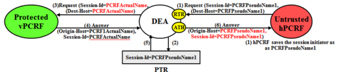
Figure 10-18 Untrusted-hPCRF to Protected-vPCRF Diameter Transaction
