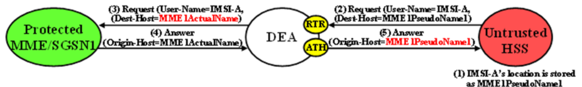
Figure 10-16 MME/SGSN TH Untrusted-HSS to Protected MME/SGSN Transaction
