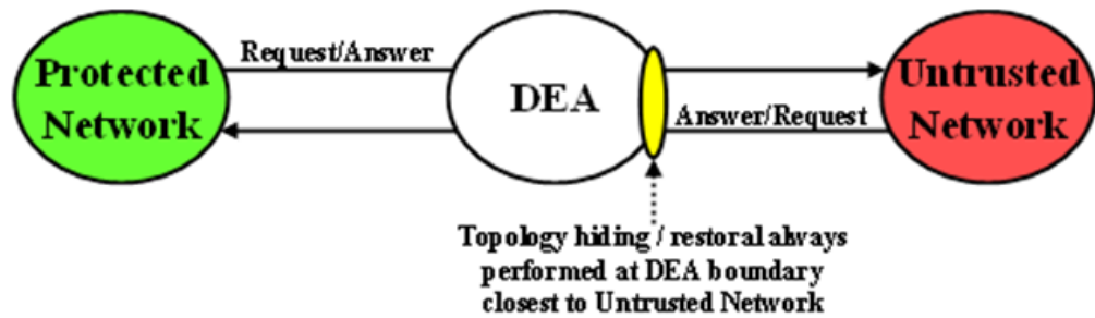
Figure 10-1 Diameter Topology Hiding Boundary
