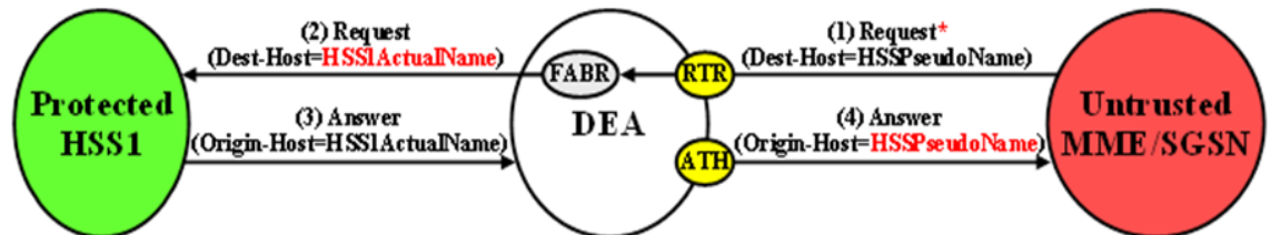
Figure 10-13 S6a/S6d HSS TH Untrusted-MME/SGSN to Protected-HSS Transaction
