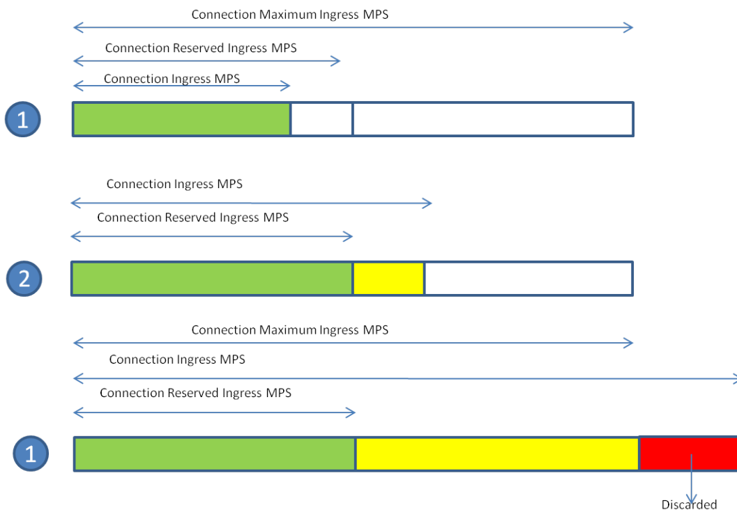
Figure 14-1 Per-Connection Message Coloring
