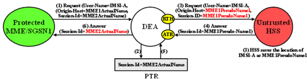
Figure 10-15 MME/SGSN TH Protected-MME/SGSN to Untrusted HSS Transaction
