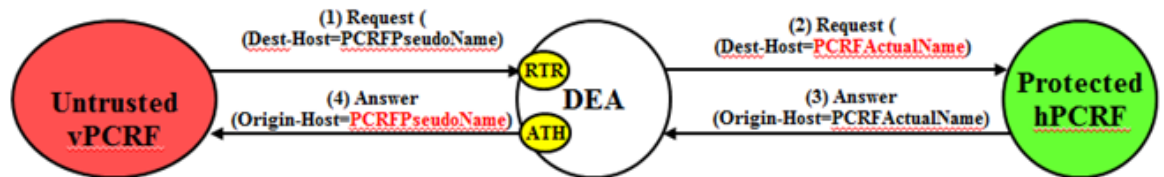
Figure 10-20 Untrusted-vPCRF to Protected-hPCRF Transaction
