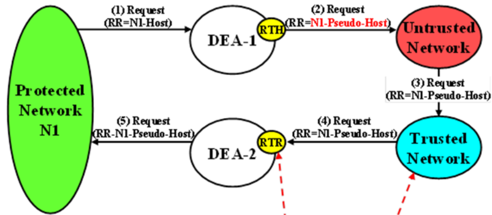
Figure 10-9 Unsupported Pseudo-Host Route-Record Loop Detection
