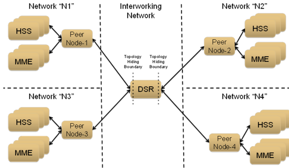
Figure 10-4 TH Network Deployment in an Interworking Network
