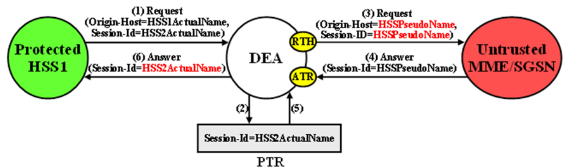
Figure 10-12 S6a/S6d HSS TH Protected-HSS to Untrusted-MME/SGSN Diameter Transaction
