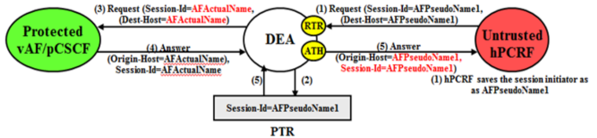
Figure 10-22 Untrusted-hPCRF to Protected-vAF/pCSCF Transaction
