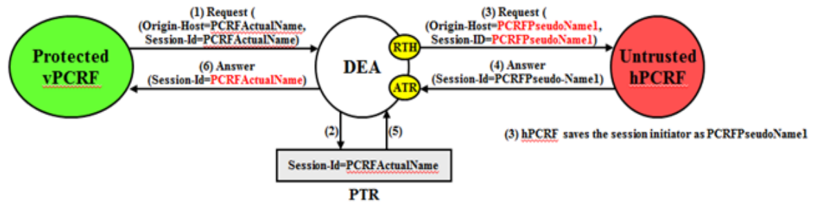
Figure 10-17 Protected-vPCRF to Untrusted-hPCRF Transaction
