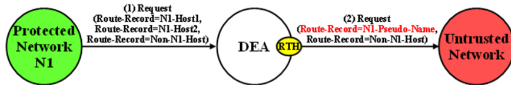
Figure 10-6 Route-Record Hiding - Request Message
