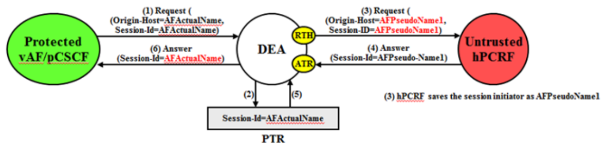
Figure 10-21 Protected vAF/pCSCF to Untrusted-hPCRF Transaction
