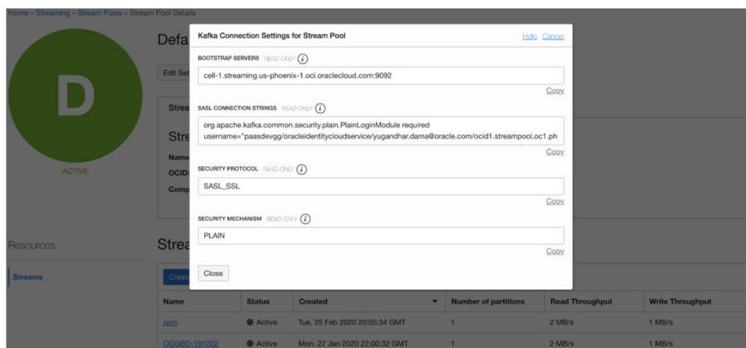
Figure 8-3 Example DefaultPool Properties
