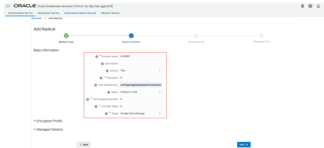
Figure 7-14 Process Name, Trail Name, and Target Names
