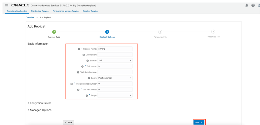
Figure 7-30 Process Name, Trail Name, and Target Names
