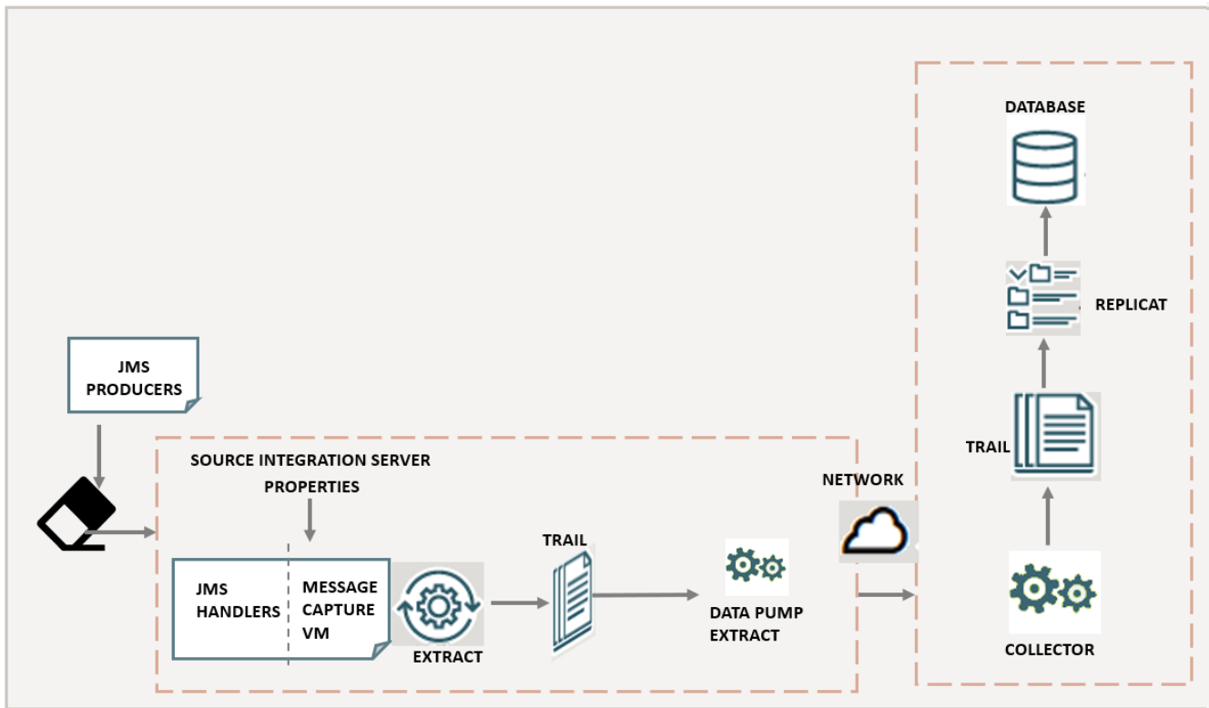
Figure 1-1 Configuration for JMS Message Capture
