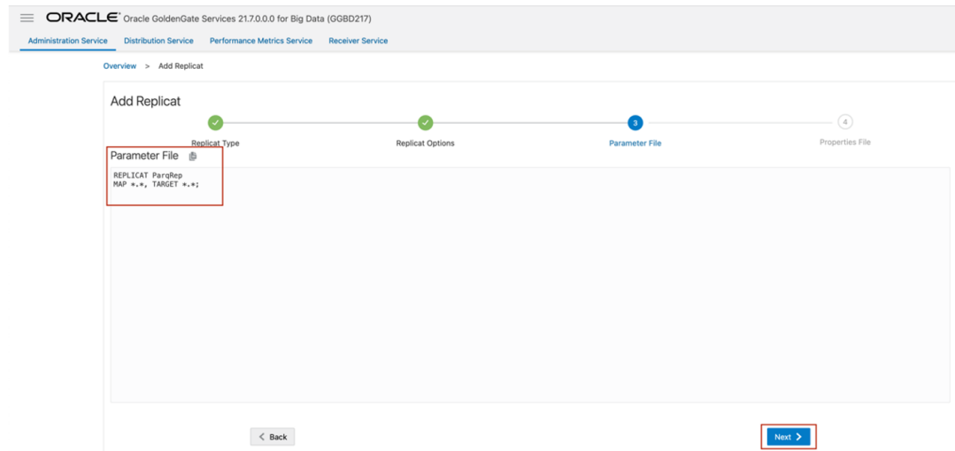
Figure 7-31 Provide Parameter File details and click Next.
