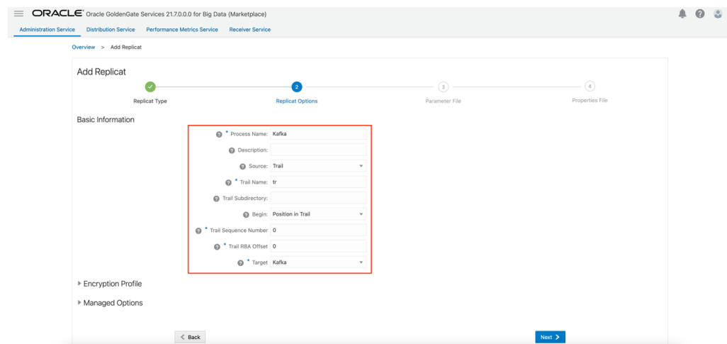
Figure 7-37 Process Name, Trail Name, and Target Names
