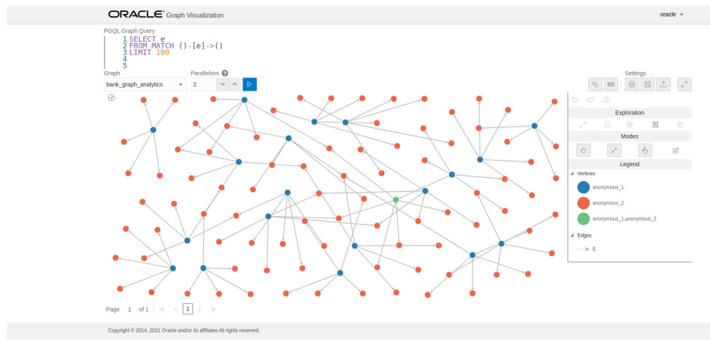
Figure 7-1 Query Visualization
