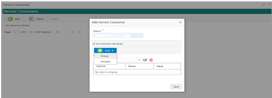
Figure 121: Environment Variables
