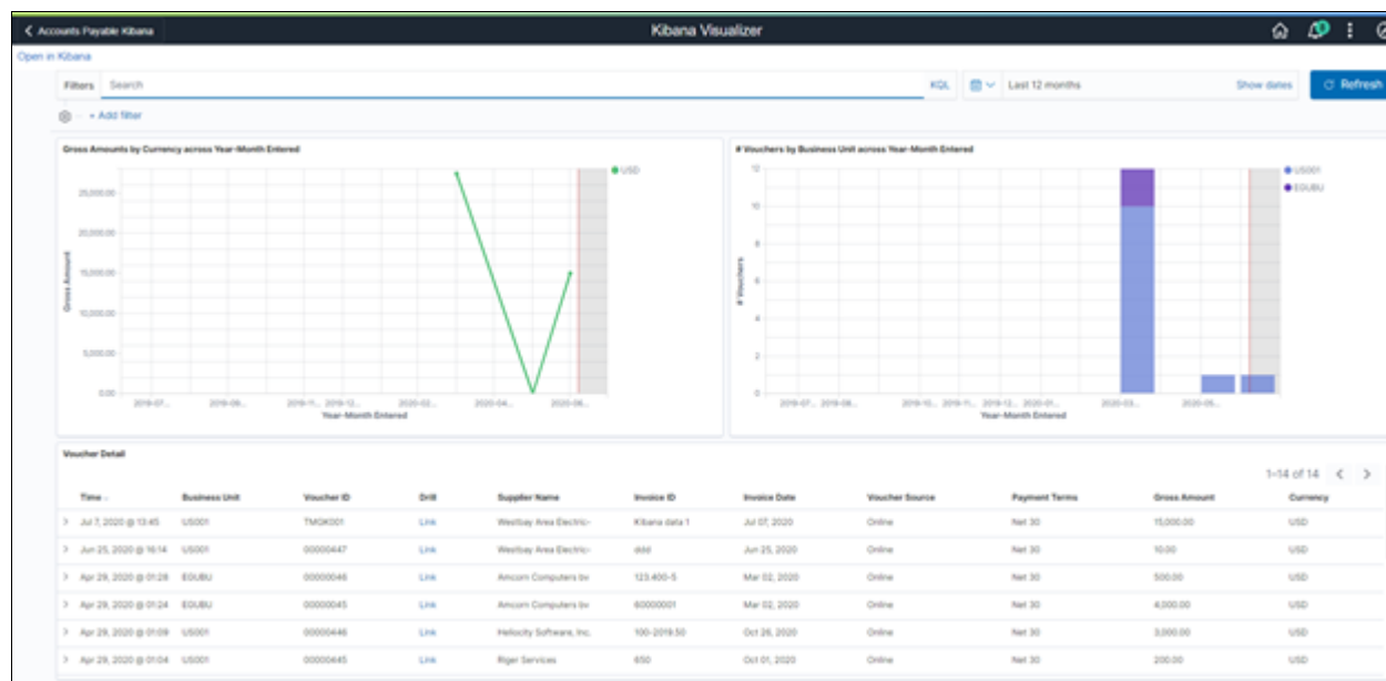
Kibana Visualizer
