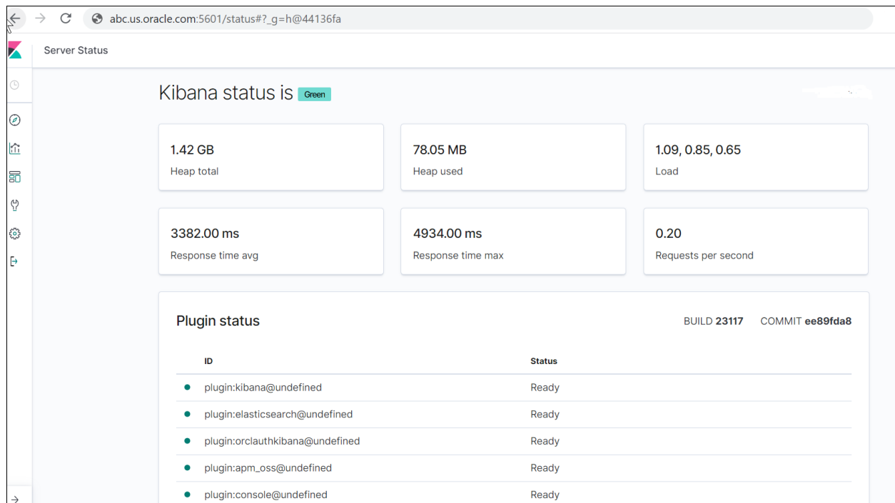
Kibana Status
