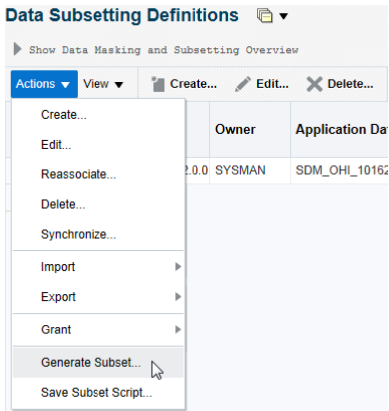
Figure 3.17: Generate Subset.
