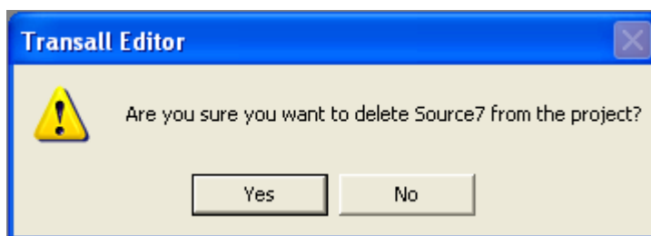
Figure 6: Delete Component
