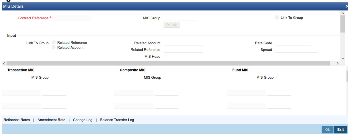
Figure 6.9: MIS Details
