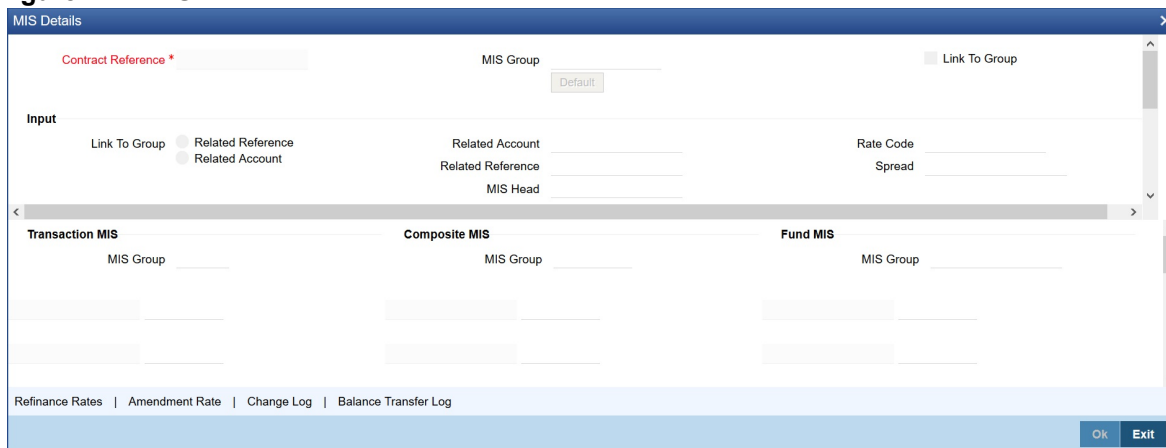
Figure 7.7: MIS
