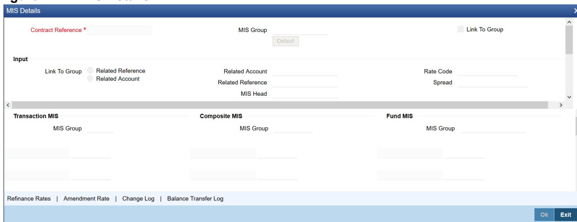
Figure 7.12: MIS Details
