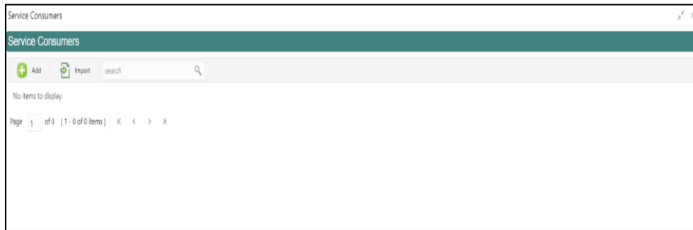
Figure 6: Service Consumers
