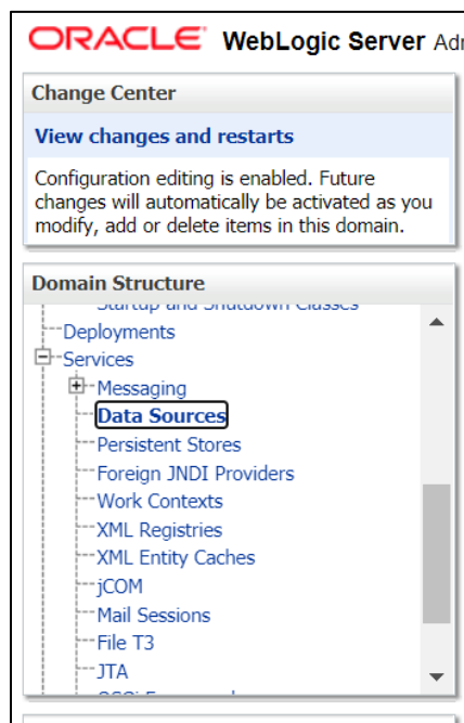
Figure 30: Data Sources
