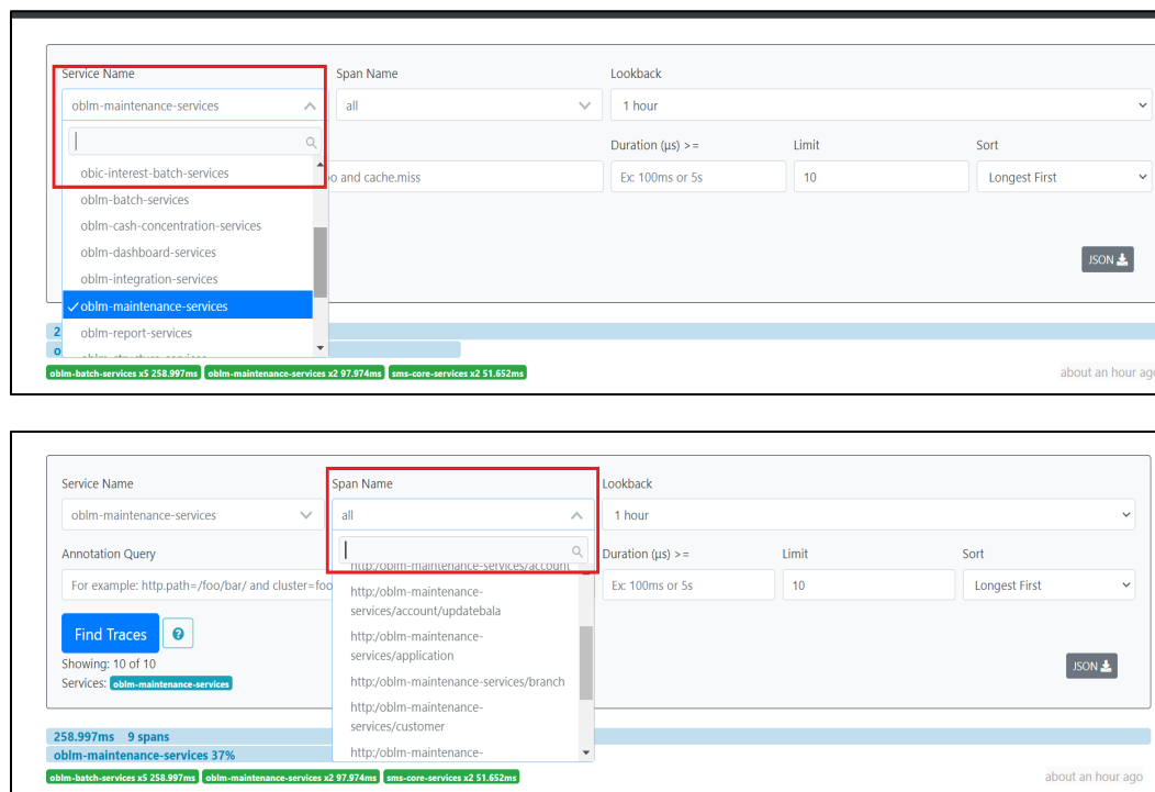
Figure 13: Find Traces
