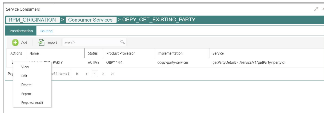
Figure 41: Service Consumers
