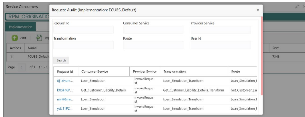
Figure 45: Request Audit
