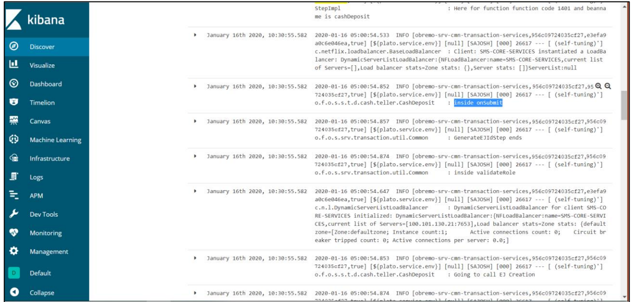
Figure 14: Accessing Kibana
