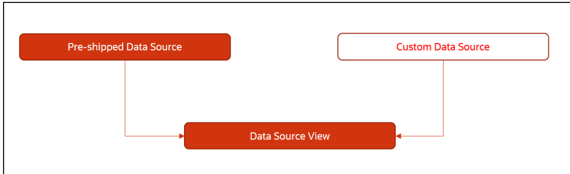
Figure 265: Data Extensibility
