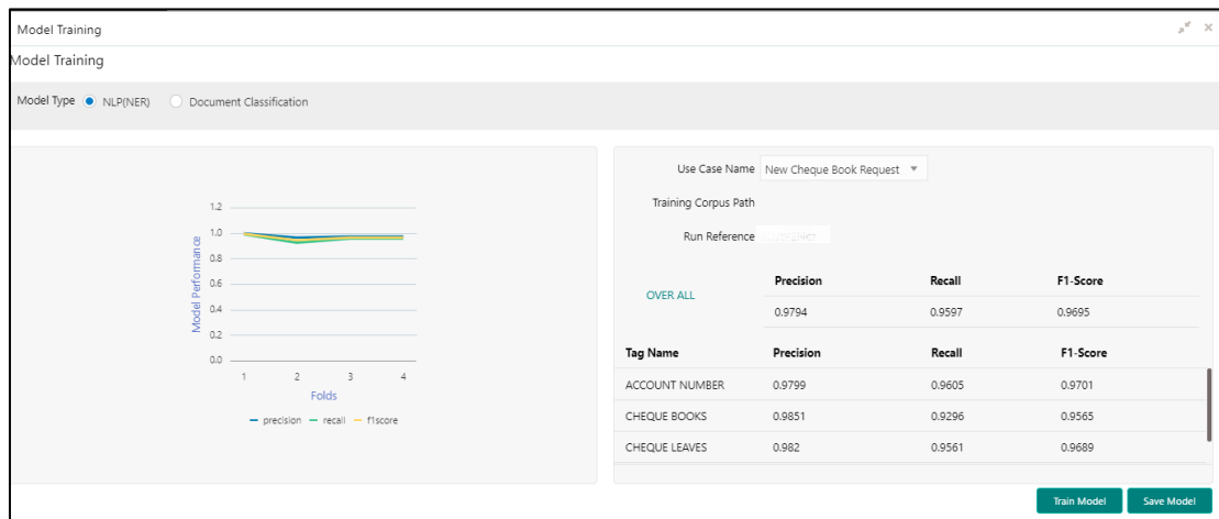
Figure 247: Model Training
