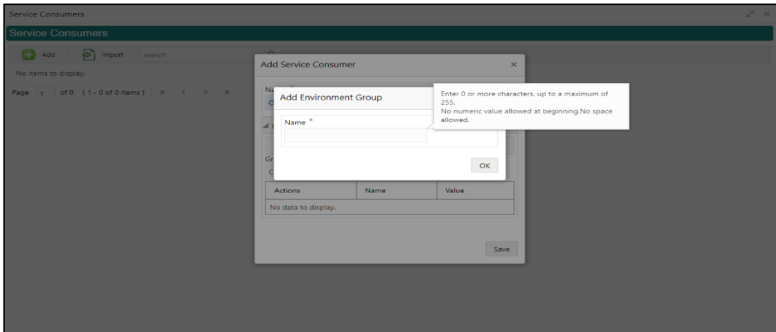
Figure 72: Environment Variables
