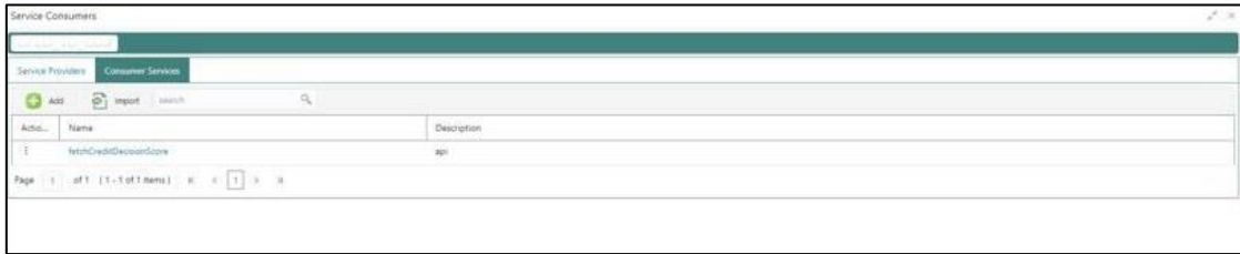
Figure 141: Consumer Services
