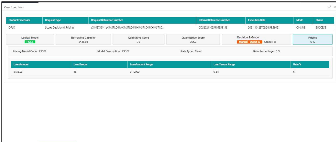
Figure 233 : Pricing Widget
