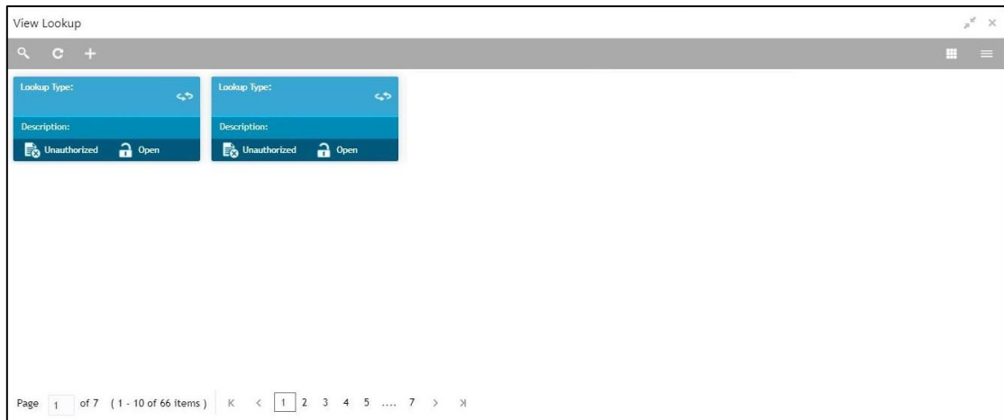
Figure 102 : View Lookup
