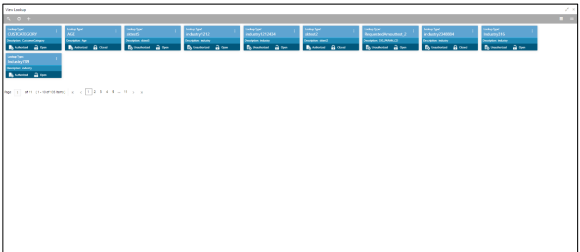
Figure 150 : View Lookup
