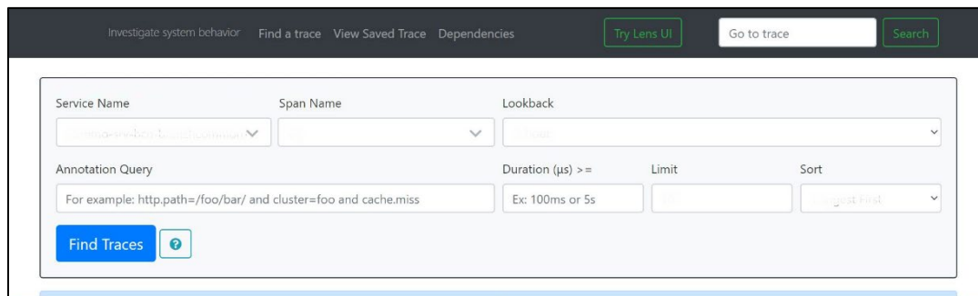
Figure 8: Find Traces
