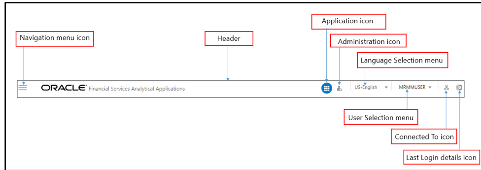
Figure 12: User Interface Components
