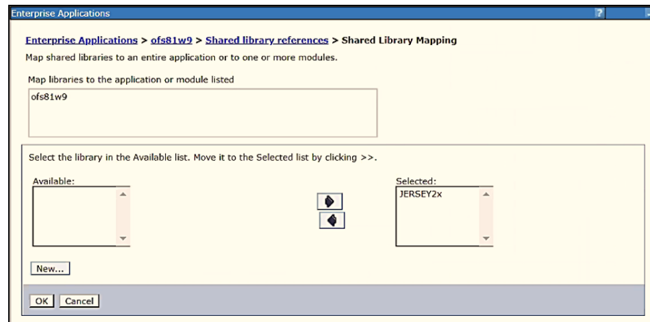
Figure 21: WebSphere Shared Libraries Mapping Selection
