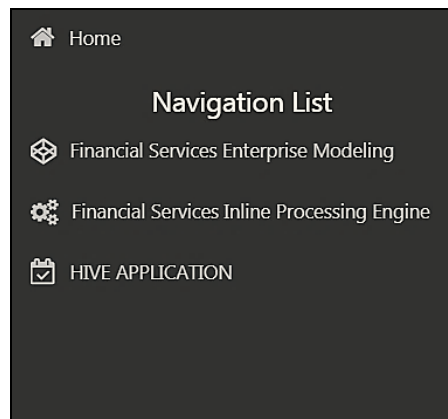
Figure 15: Navigation Drawer
