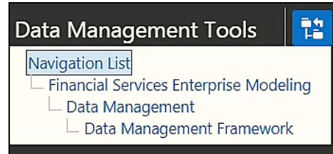
Figure 17: Navigation Submenu
