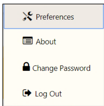
Figure 13: User Menu
