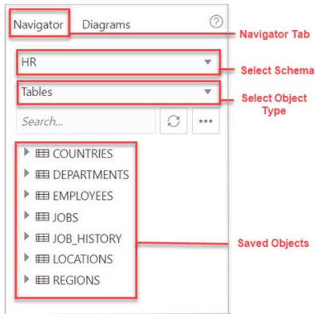
Figure 3-12 Navigator Tab
