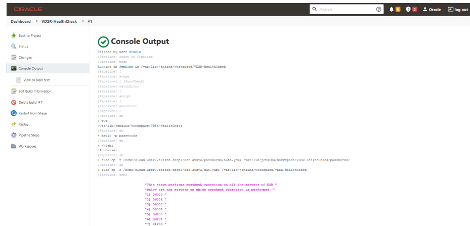
Figure 3-5 Console Output
