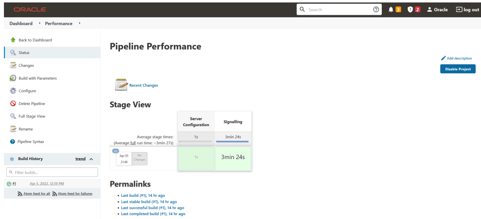
Figure 3-7 Performance Build
