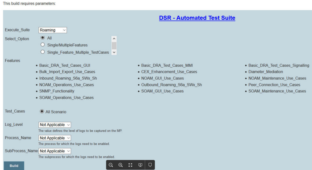
Figure 3-6 Regression Parameters
