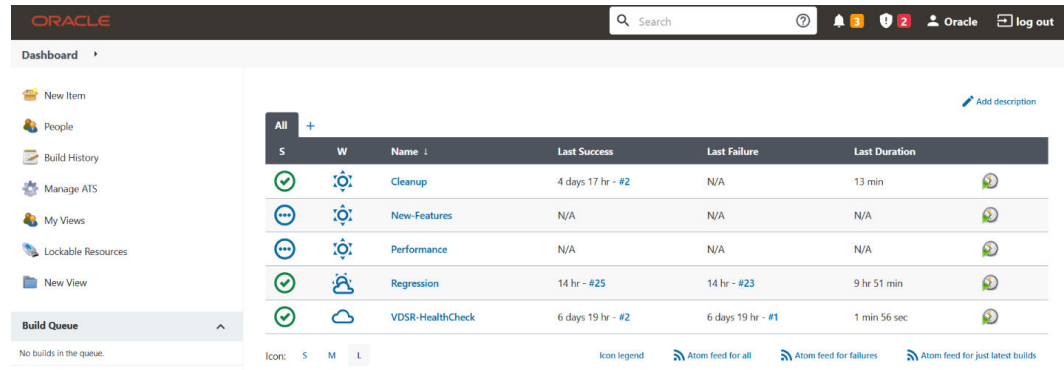
Figure 3-4 Jenkins GUI
