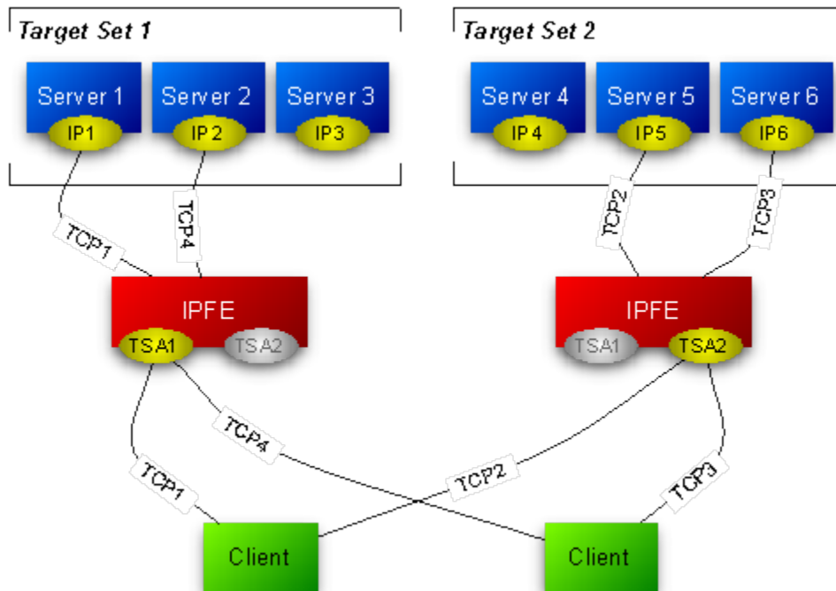
Figure 2-1 IPFE Architecture
