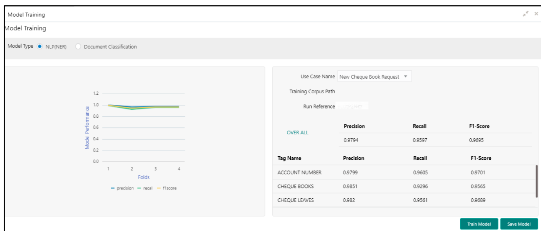
Figure 245: Model Training
