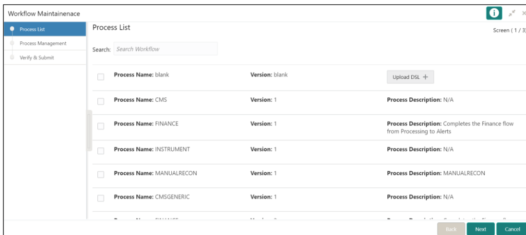
Figure 9: Process List
